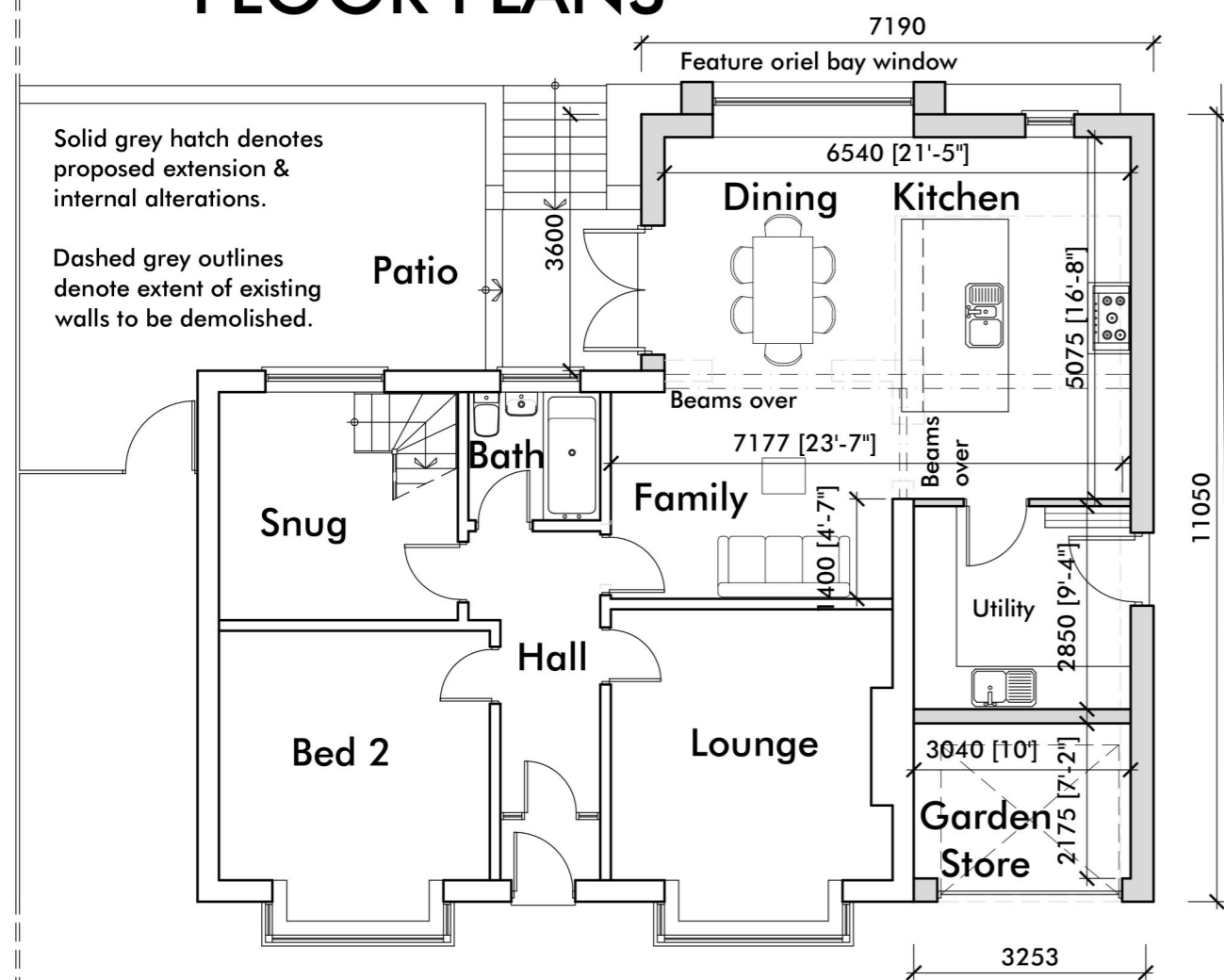
GROUND FLOOR
