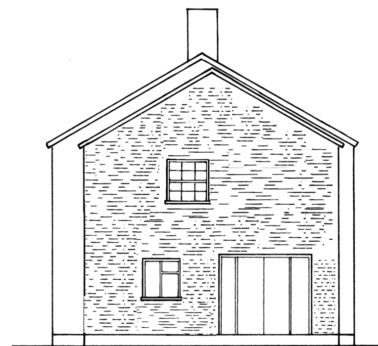
SIDE ELEVATION
