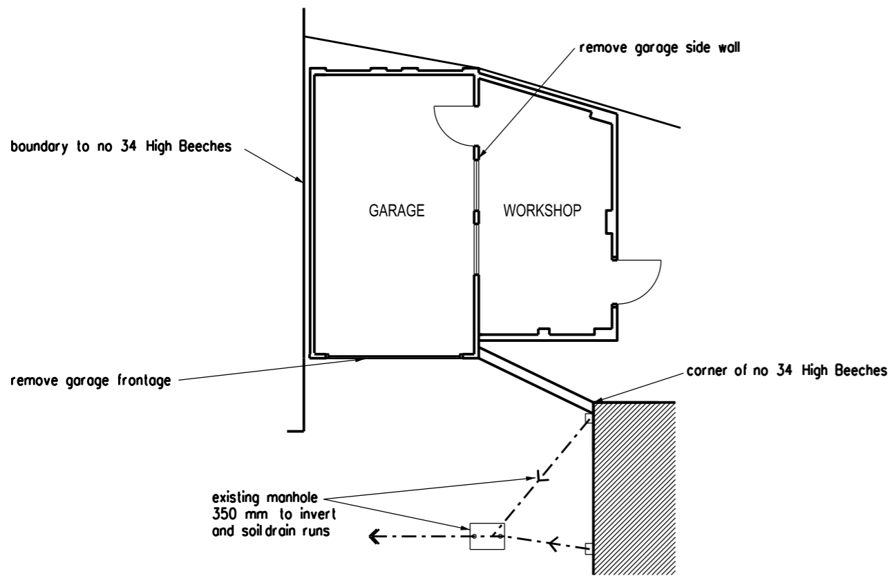
GARAGE PLAN
