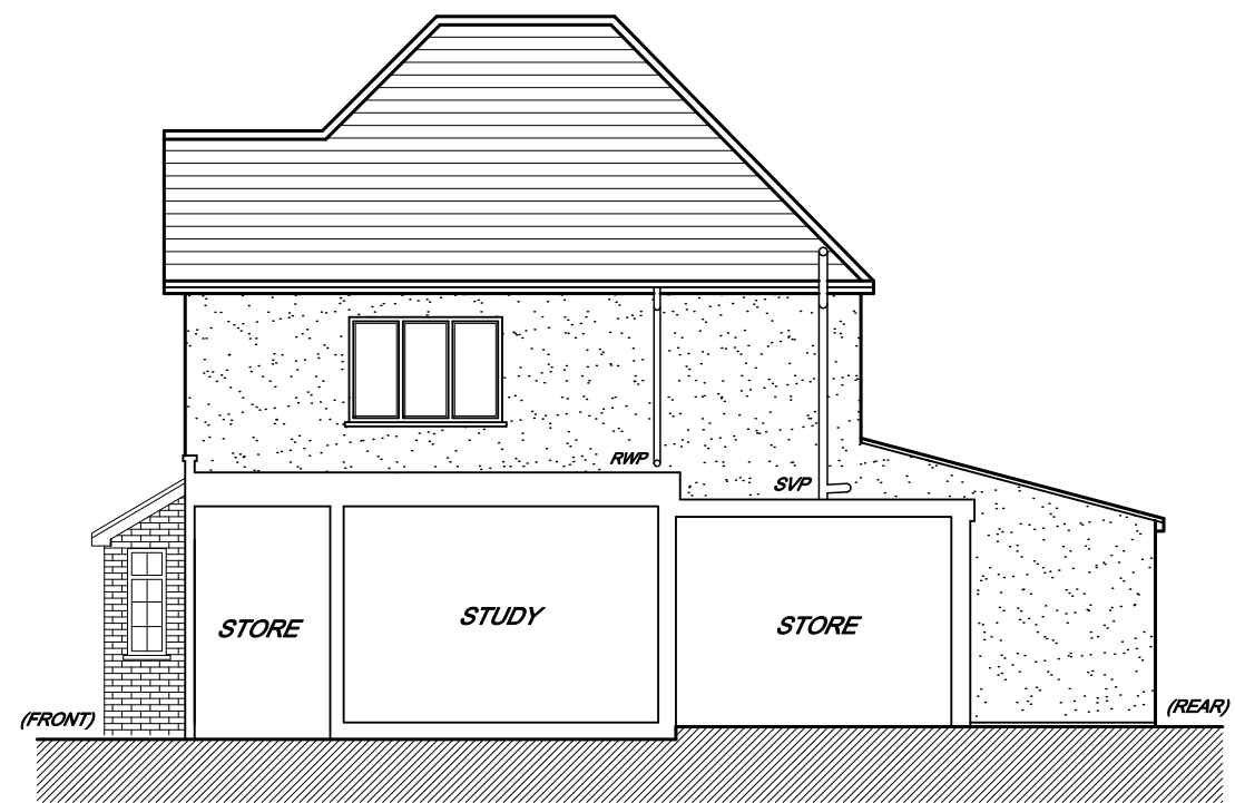
PROPOSED SECTION THROUGH BUILDING
