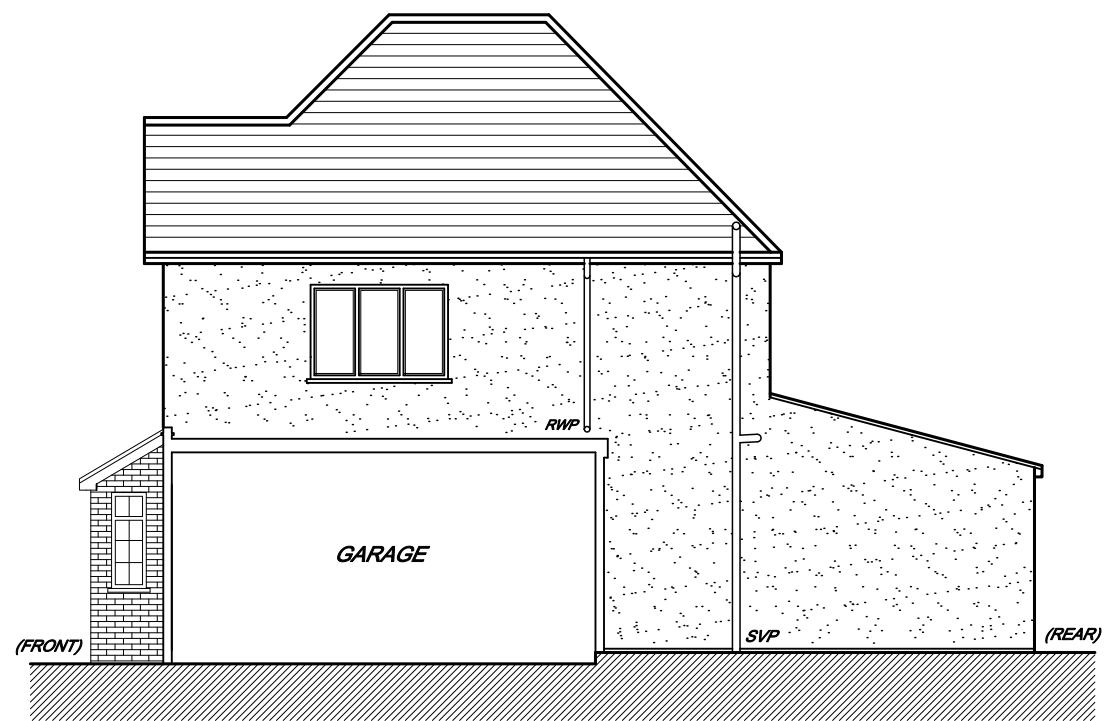
EXISTING SECTION THROUGH BUILDING
