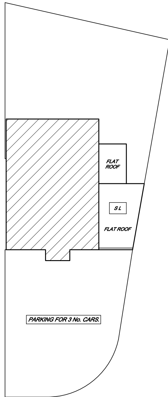
SITE / ROOF PLAN SCALE - 1:200.
