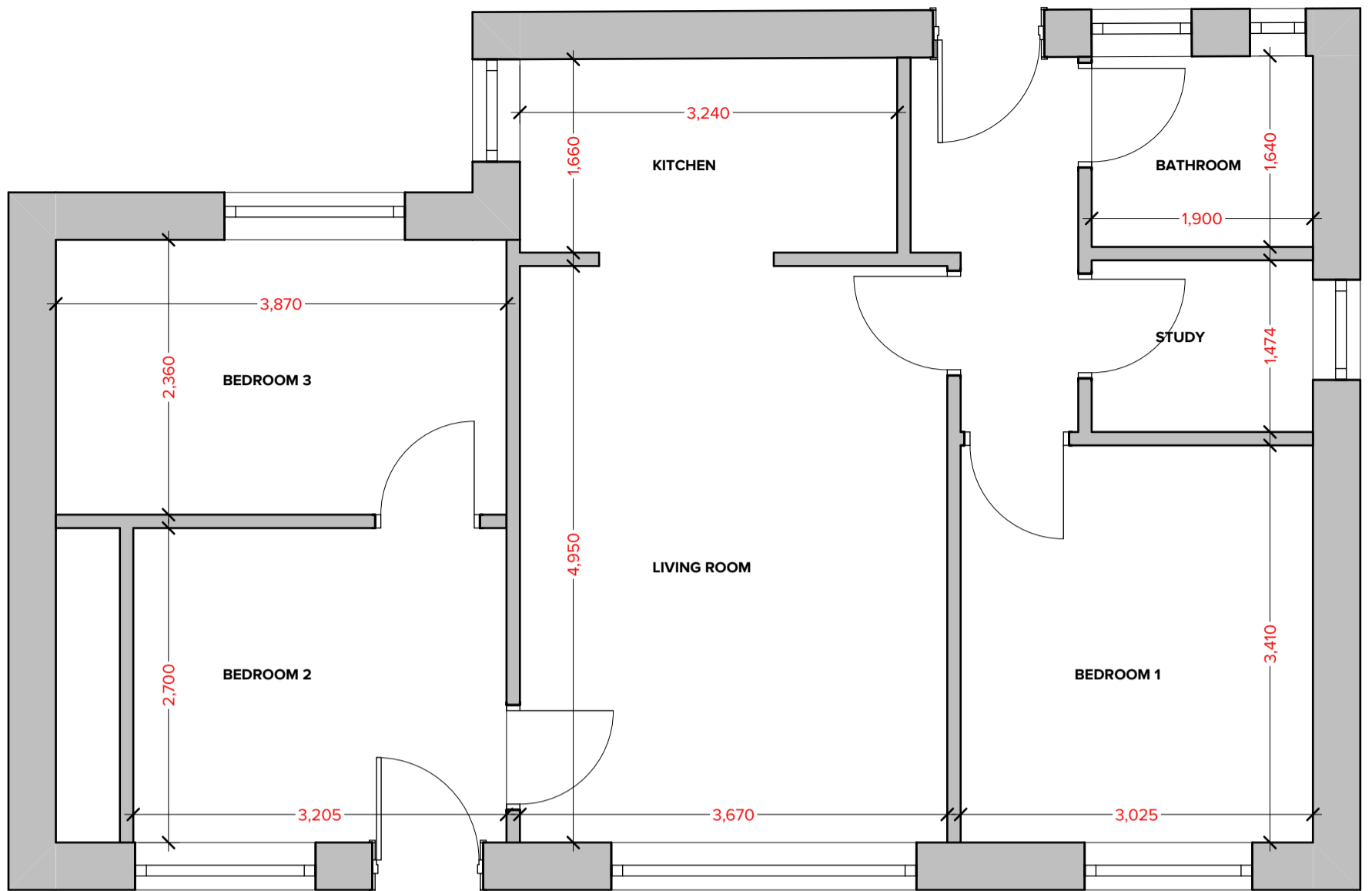
EXISTING PLAN 1:50
