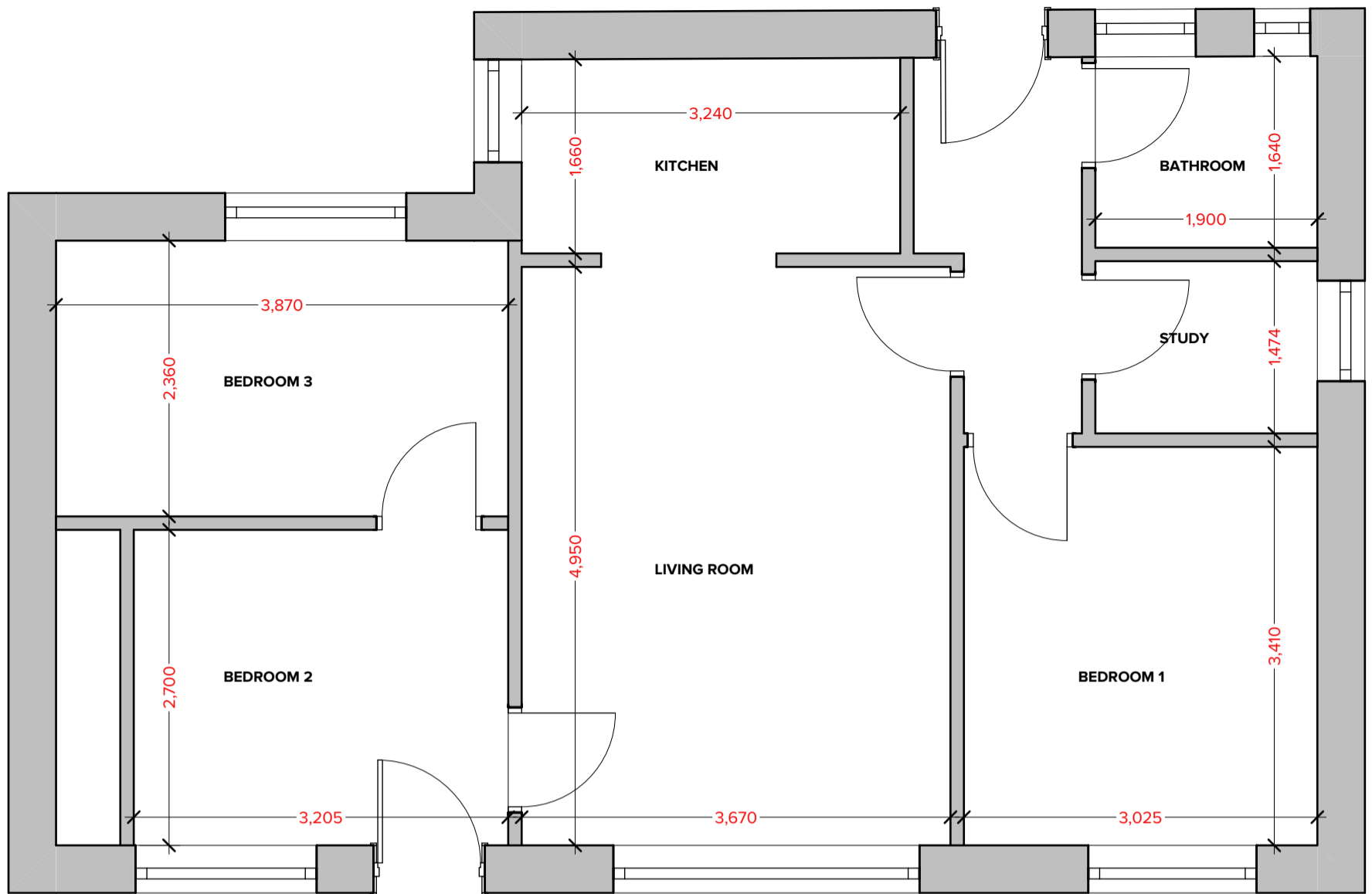
EXISTING PLAN 1:50
