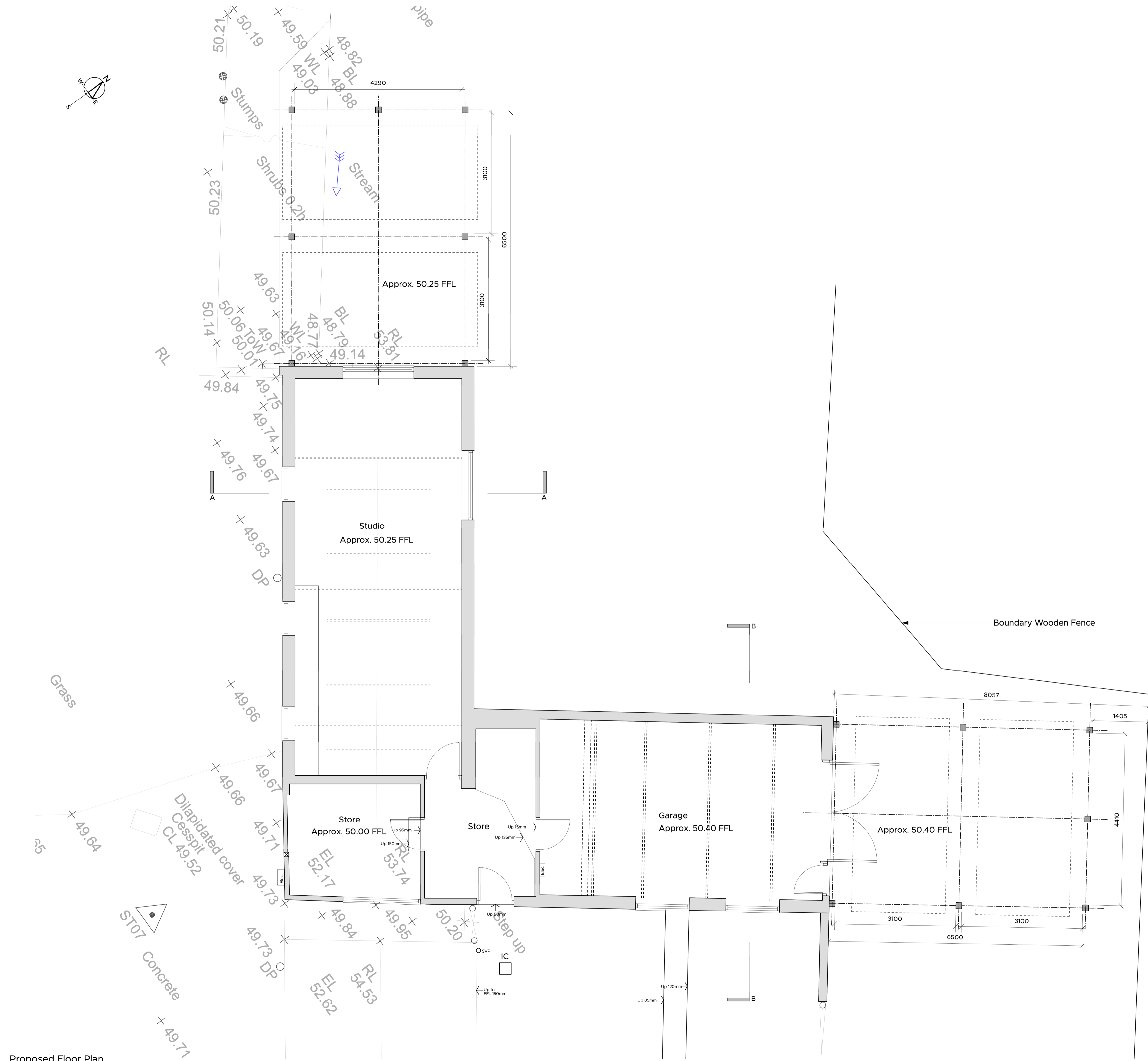
Proposed Floor Plan Scale: 1:50
