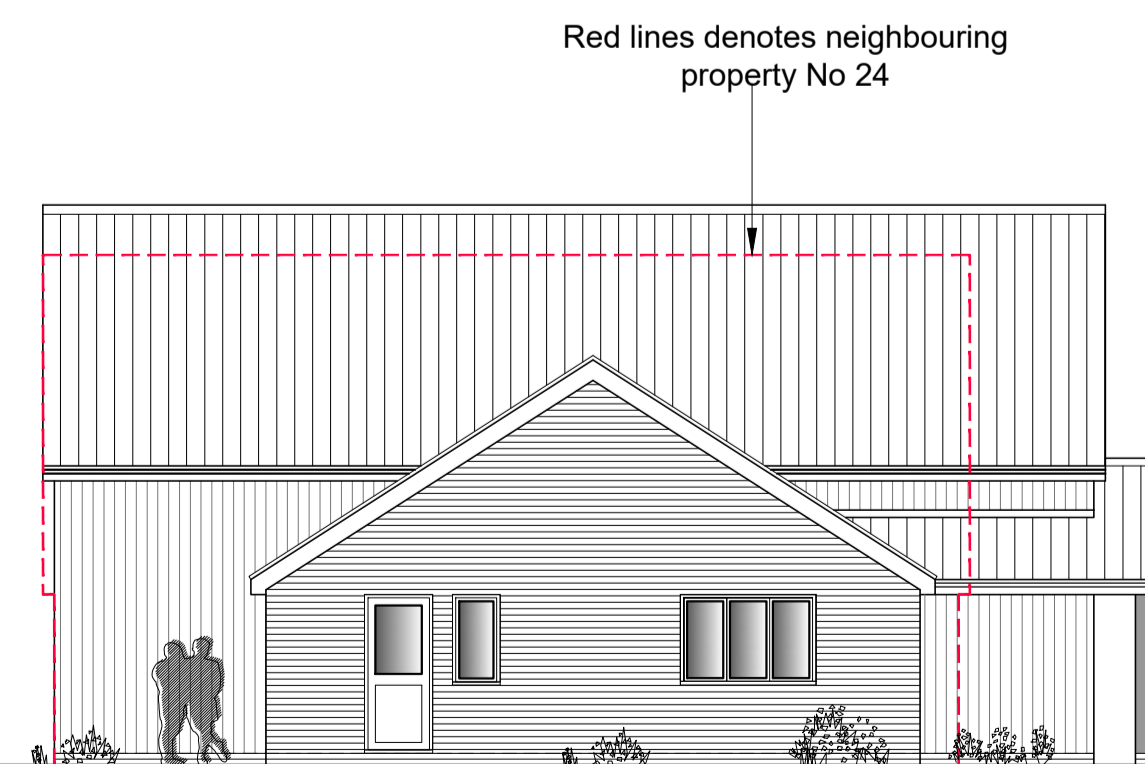
1:100 Proposed Side Elevation (South)
