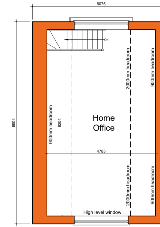
1:50 Proposed First Floor Plan
