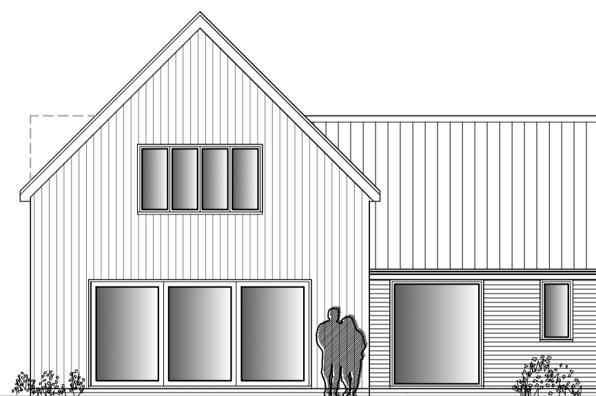
1:100 Proposed Rear Elevation (West)
