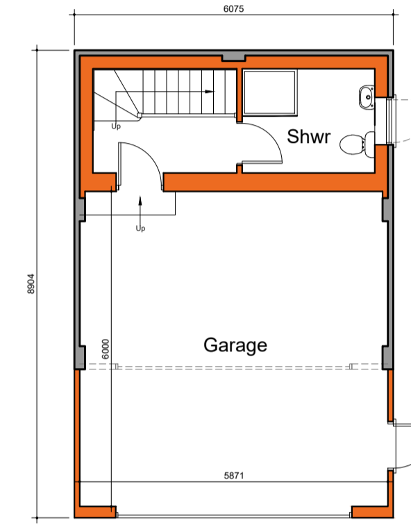
1:50 Proposed Ground Floor Plan
