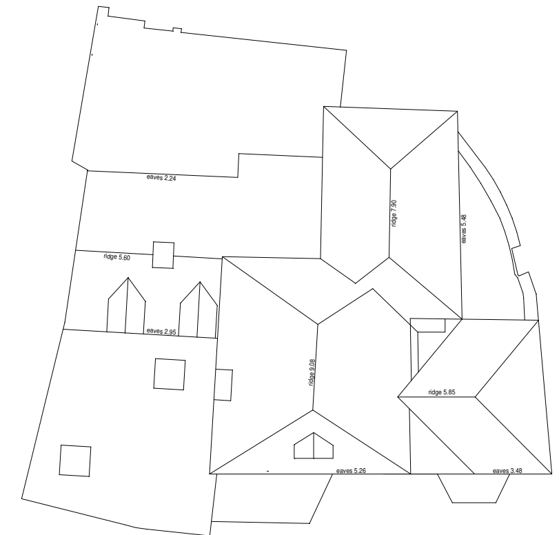
ROOF PLAN
