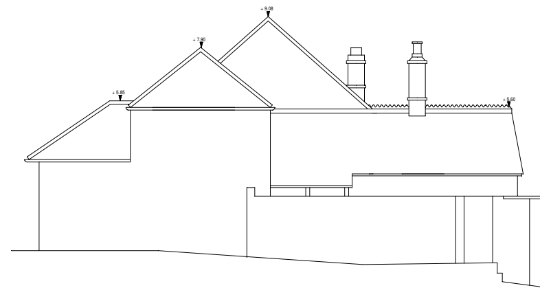
REAR ELEVATION
