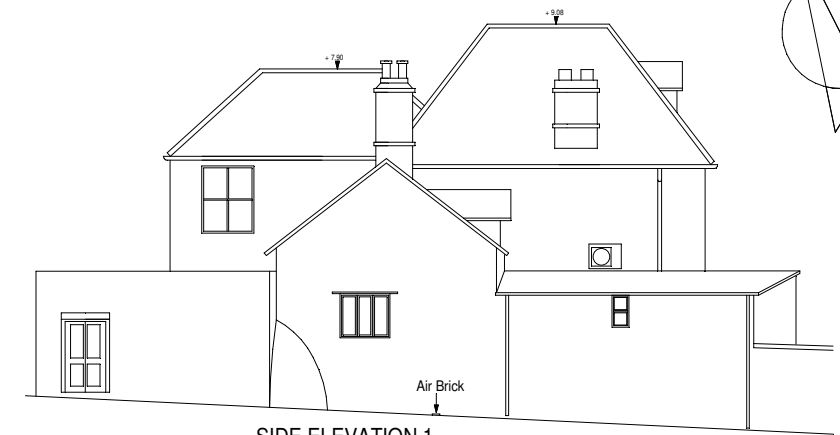
SIDE ELEVATION 1
