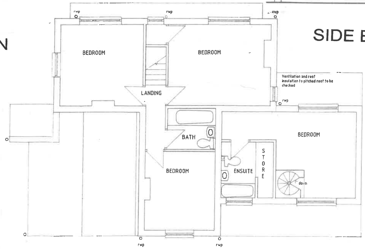
FIRST FLOOR
