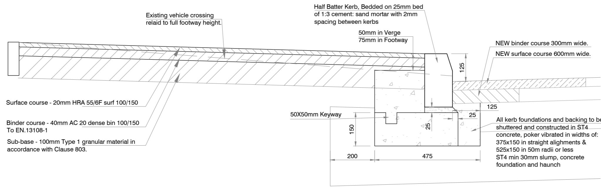
Footway Construction
