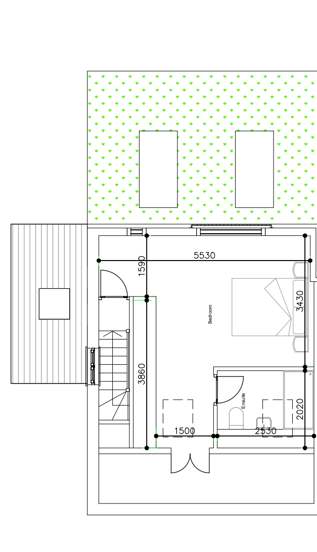
Proposed Loft Floor Plan
