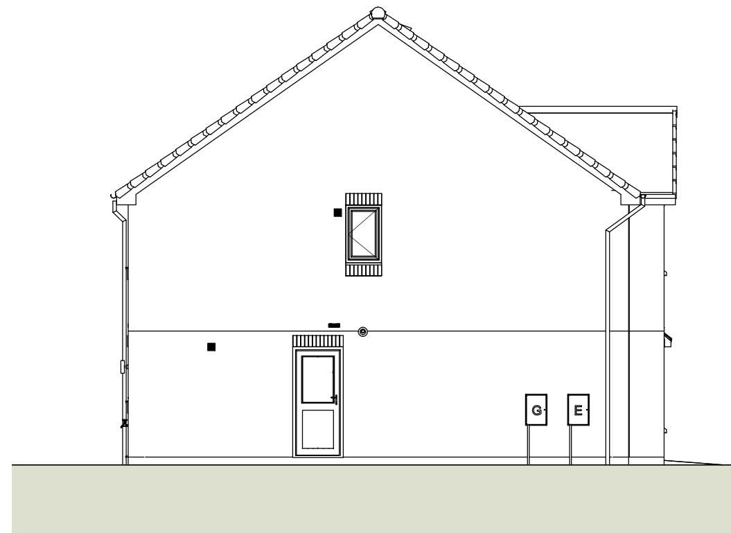
Side Elevation
