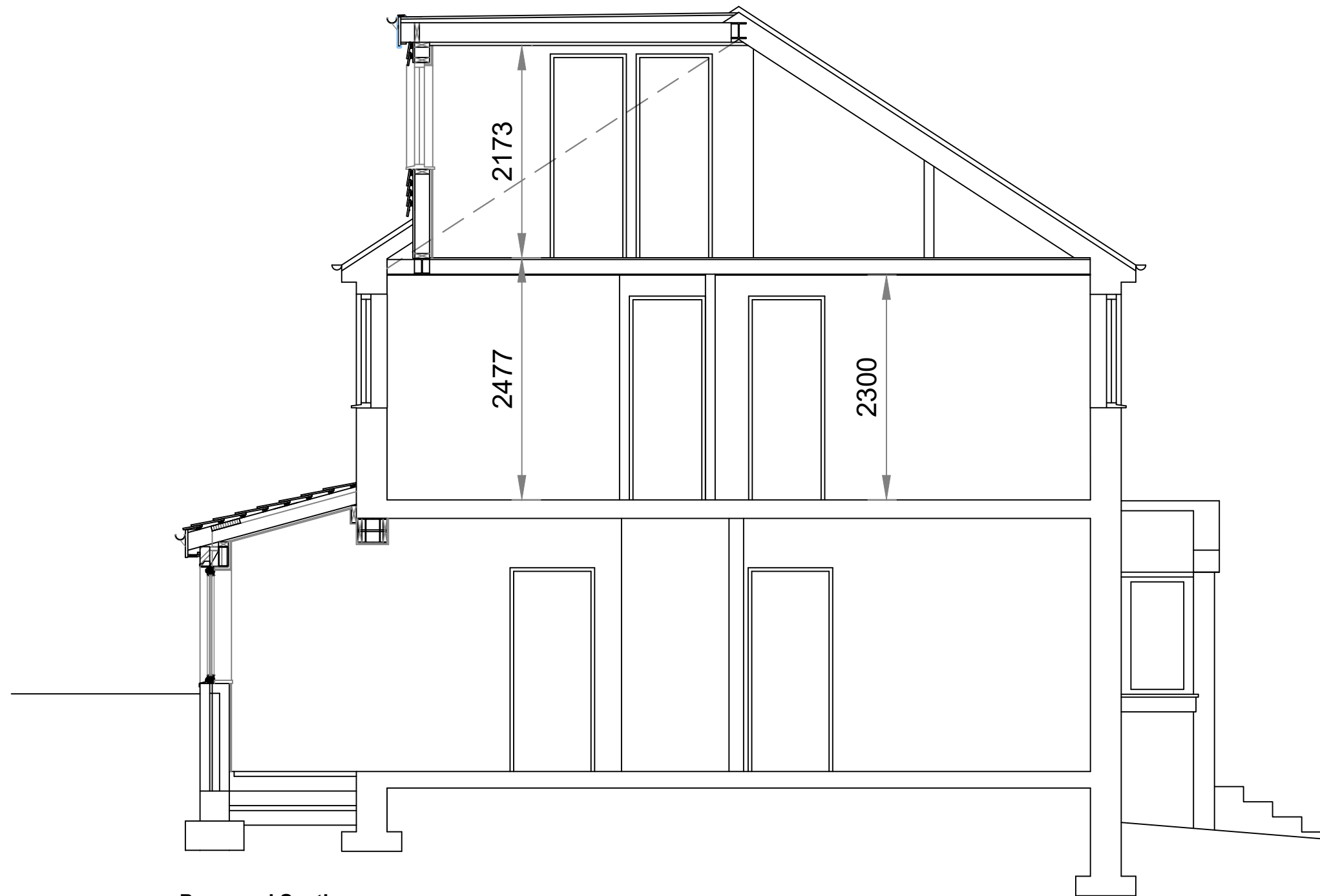
Proposed Section
