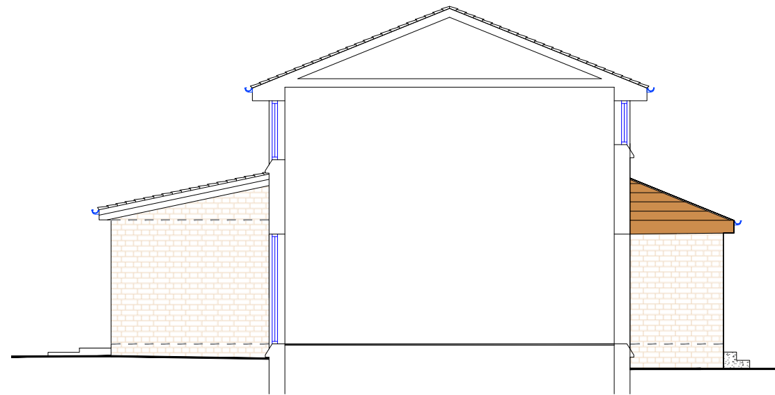
Side Elevations (West Facing) Front and Rear Extensions Scale: 1/100 @ A3
