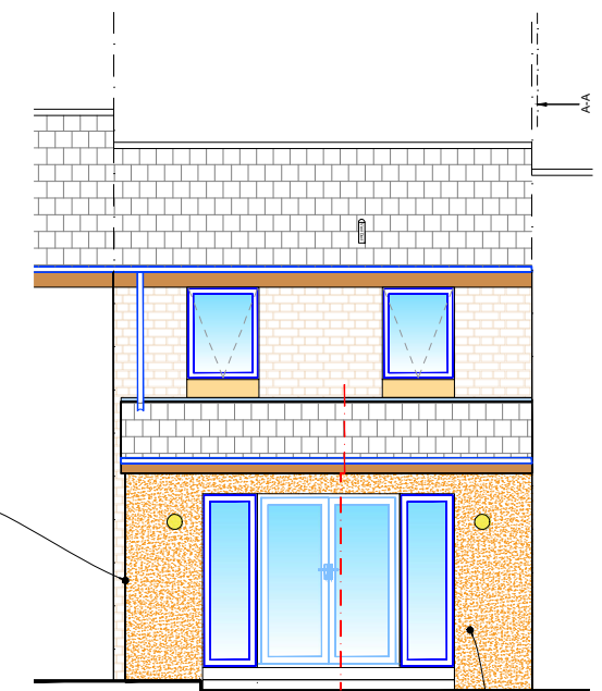
Rear Elevation as Proposed Scale: 1/100 @ A3
