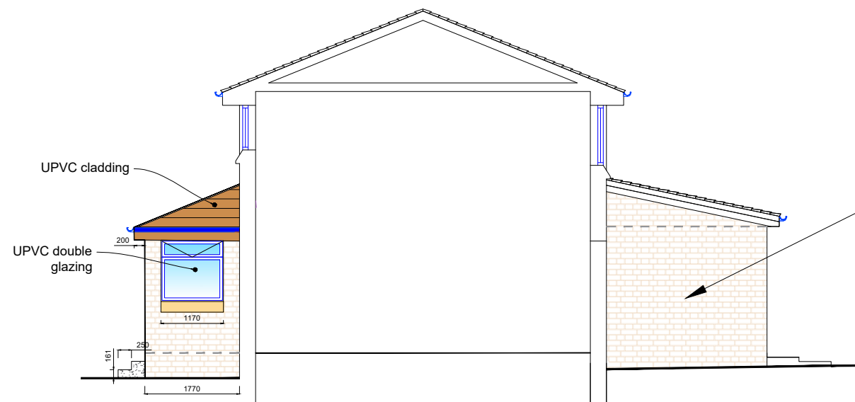
Side Elevation (East Facing) Front and Rear Extensions Scale: 1/100 @ A3
