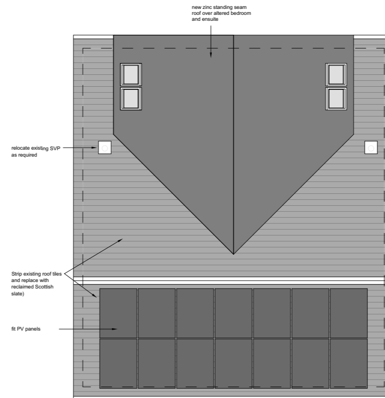
Proposed Roof Plan 1:100 @ A3
