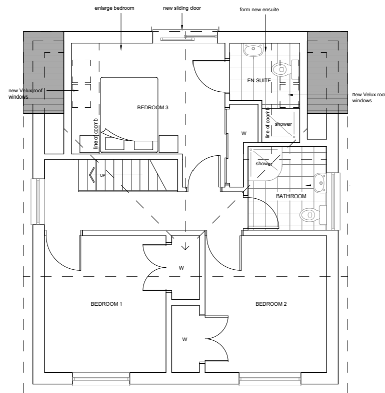
Proposed First Floor Plan 1:100 @ A3
