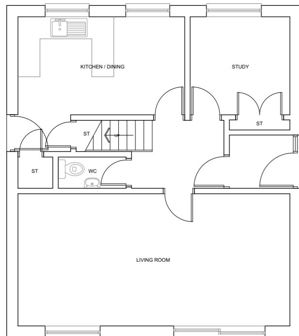
Existing Ground Floor Plan 1:100 @ A3
