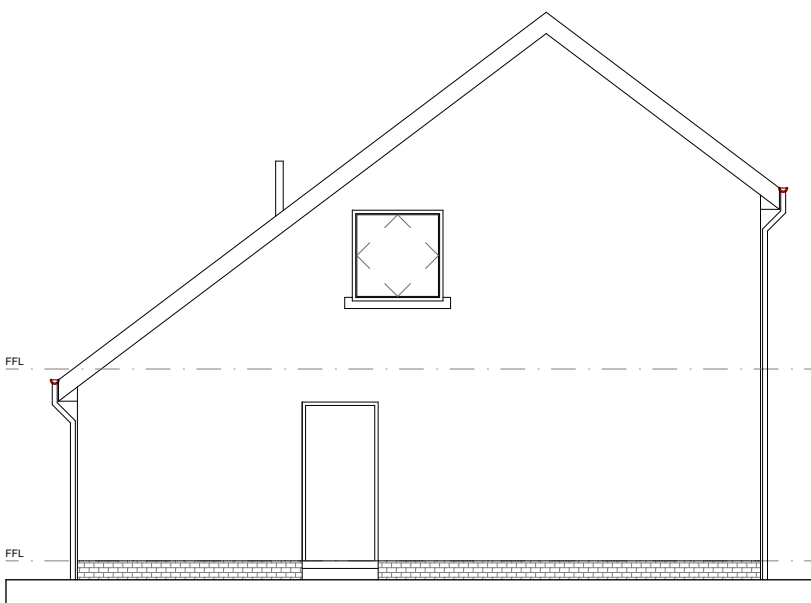
Existing West Elevation 1:100 @ A3
