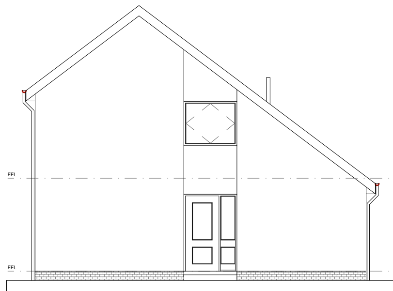
Existing East Elevation 1:100 @ A3
