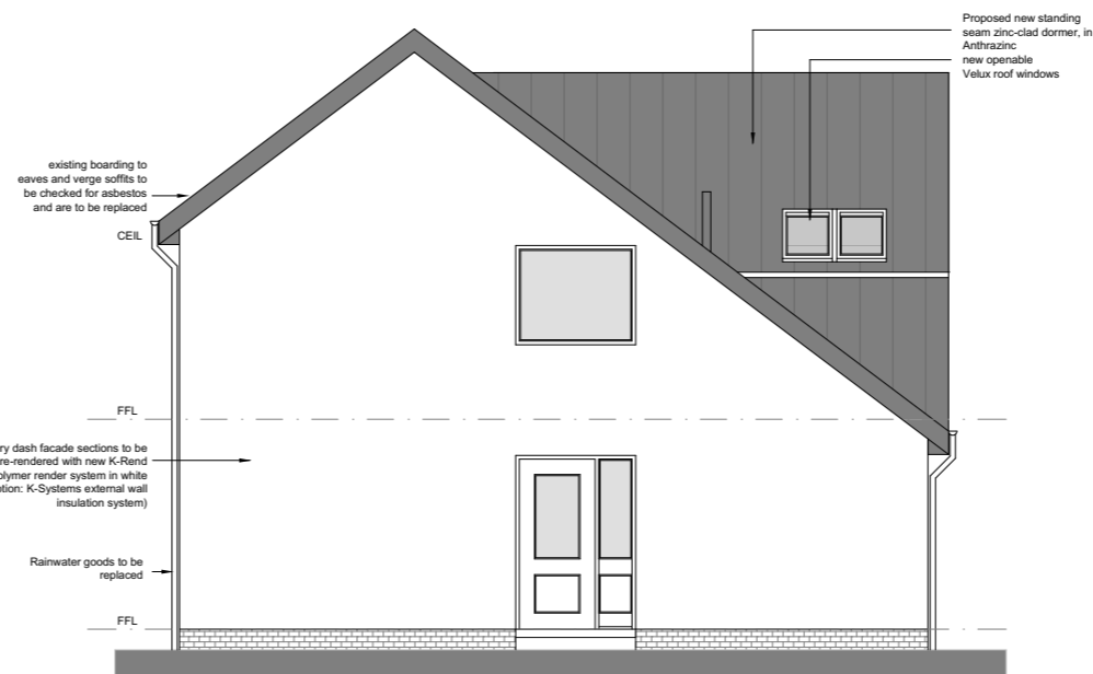
Proposed East Elevation 1:100 @ A3
