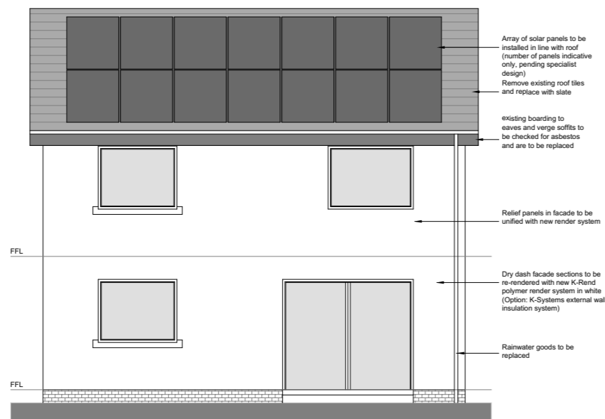
Proposed South Elevation 1:100 @ A3
