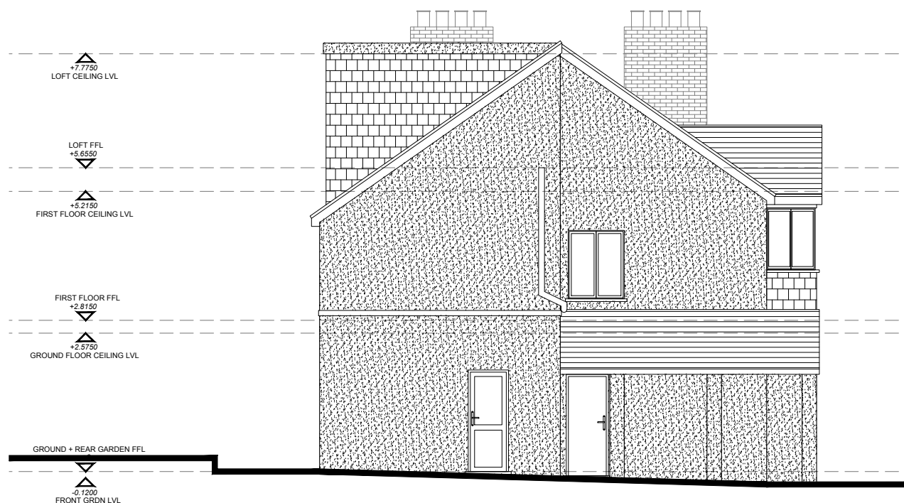
SIDE ELEVATION 01
