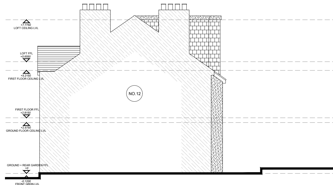
SIDE ELEVATION 02
