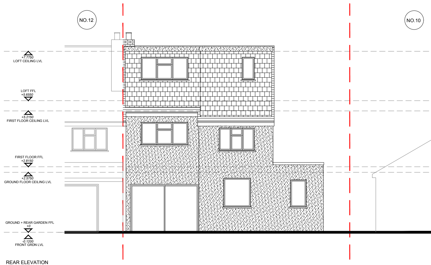
REAR ELEVATION
