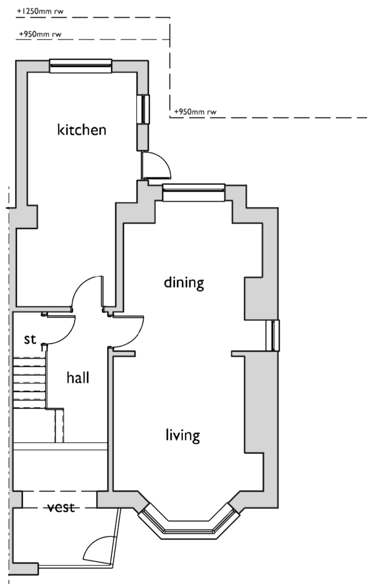
04 Ground Floor Layout I:100
