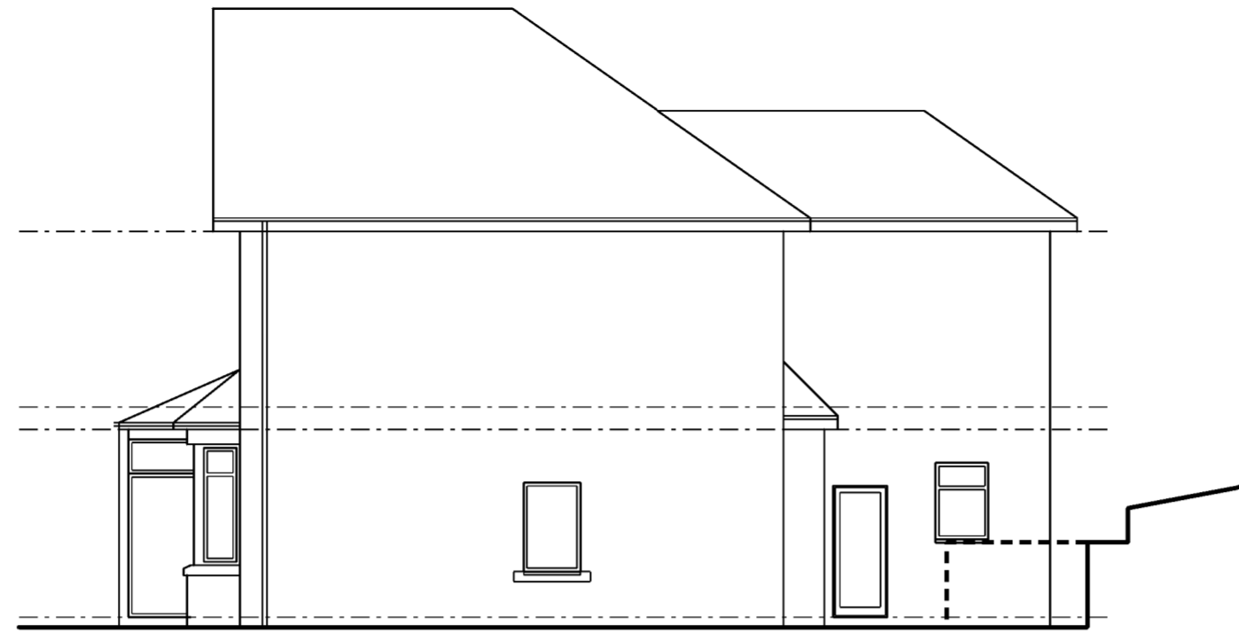
02 Side (East) Elevation I:100
