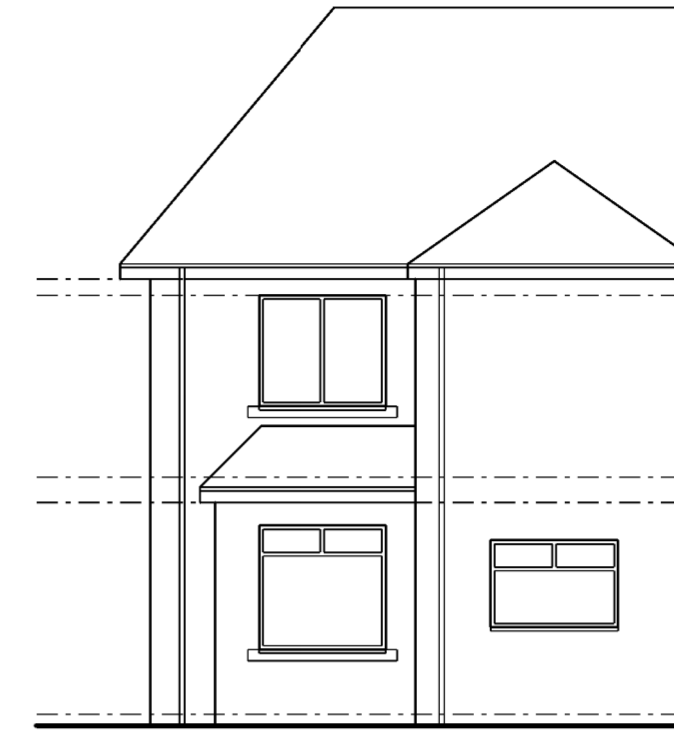
03 Rear (North) Elevation I:100
