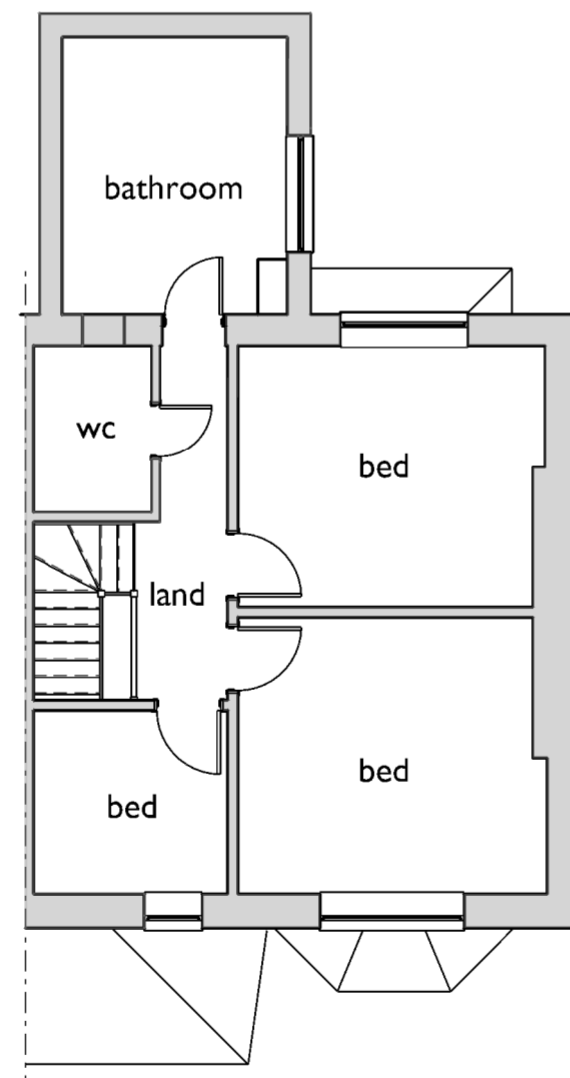
05 First Floor Layout I:100
