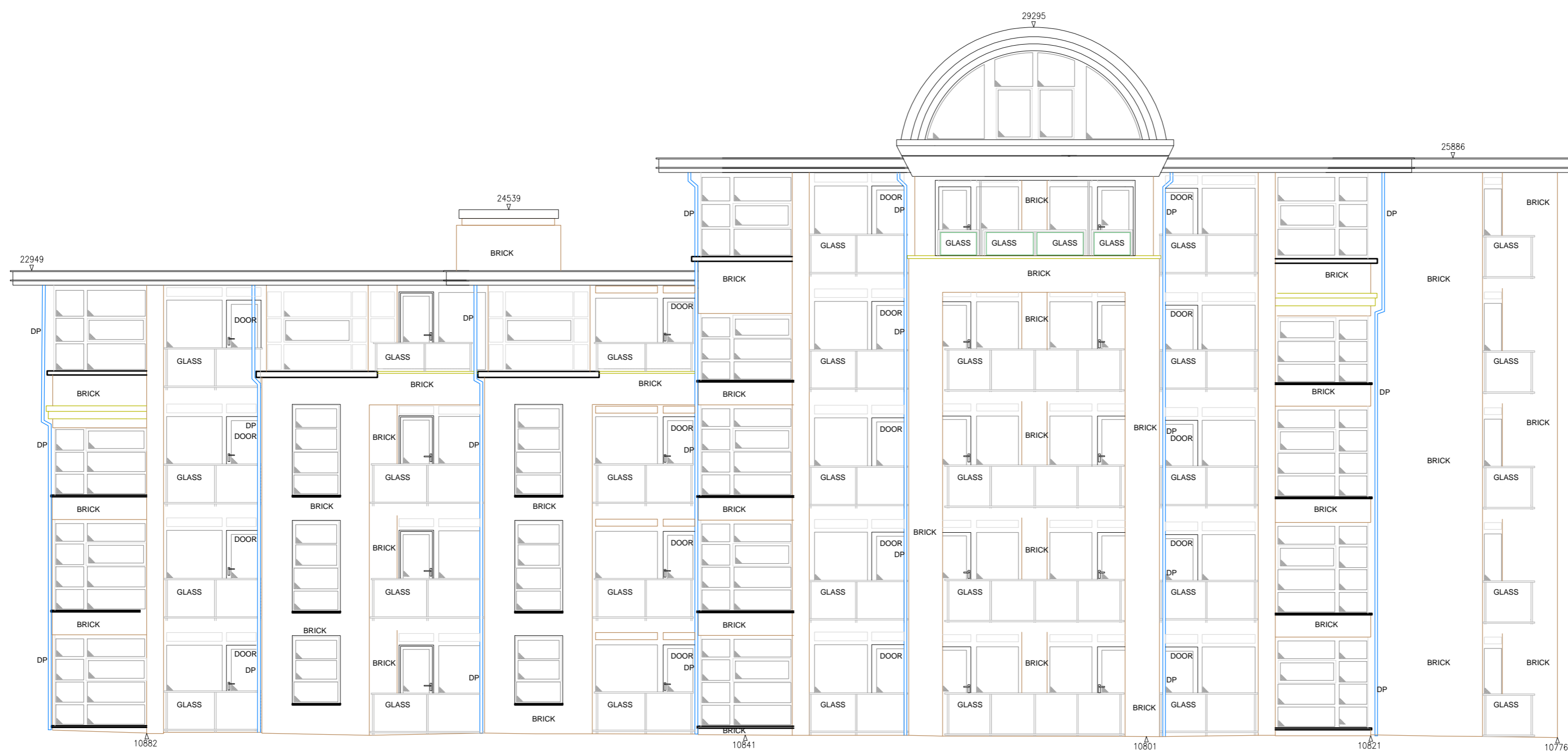
West Elevation Proposed
