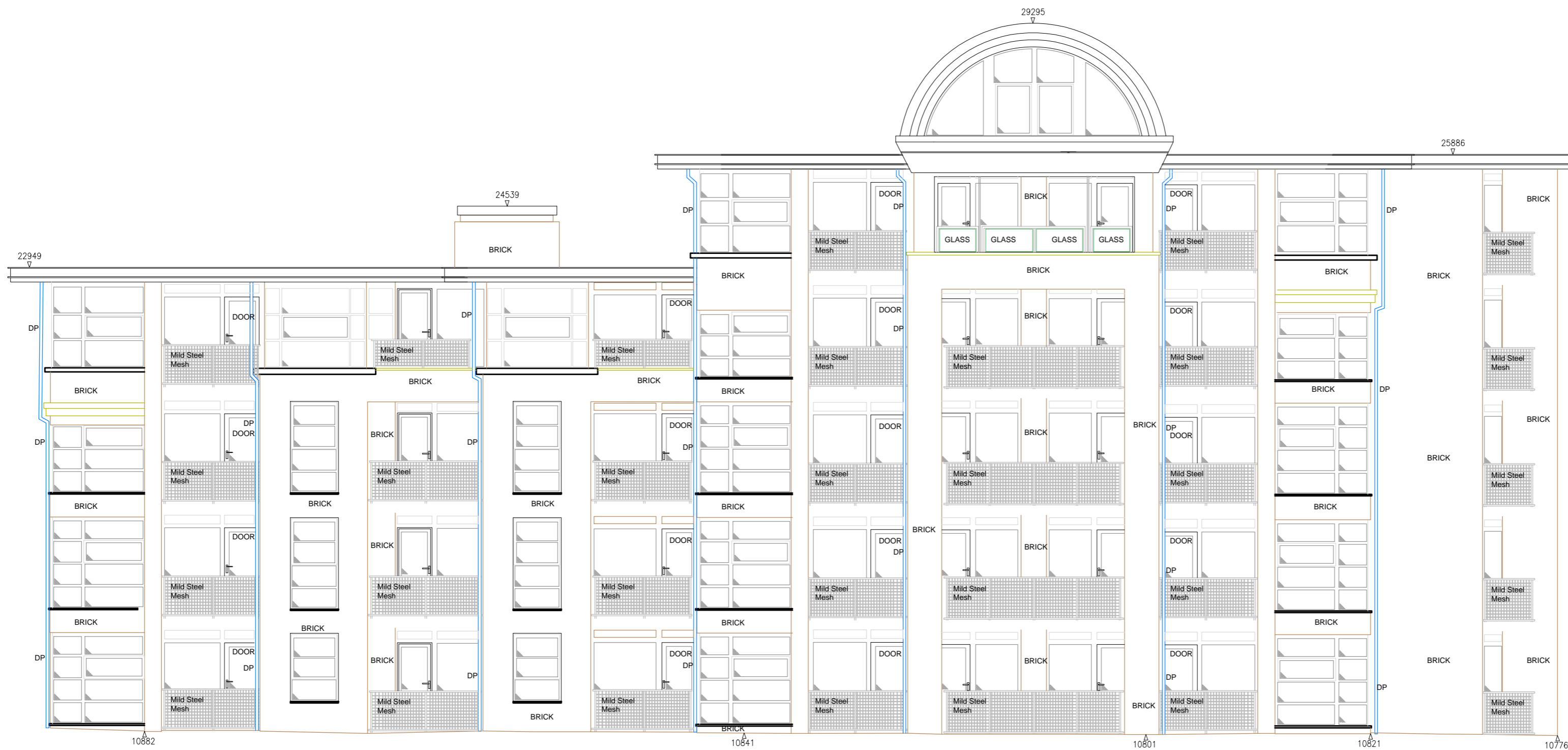
West Elevation as Existing
