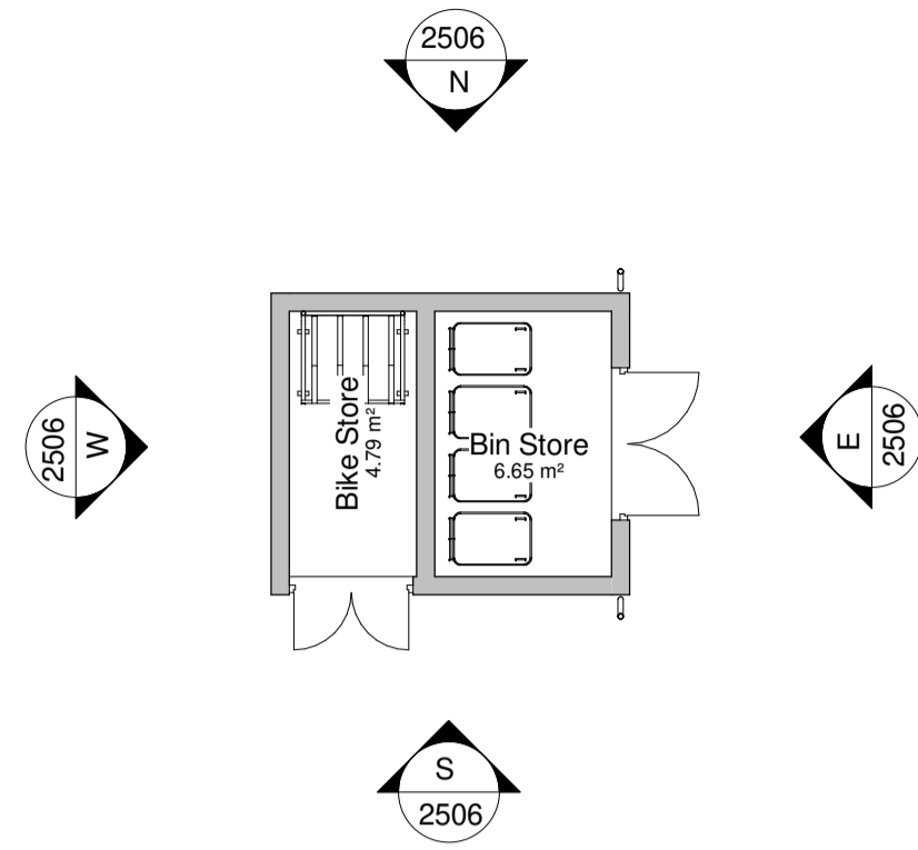
Ground Floor Proposed Plan
