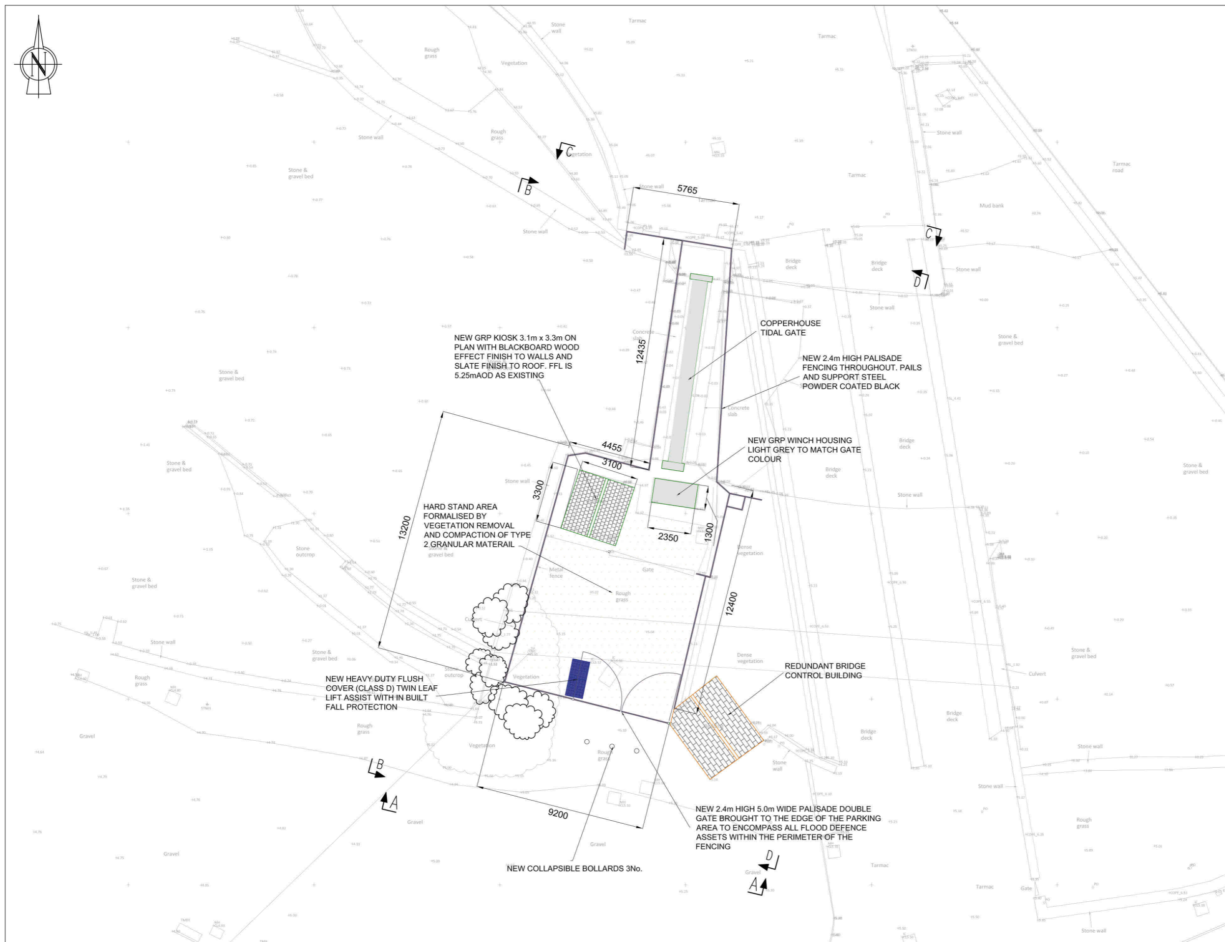
COPPERHOUSE GATE PROPOSED PLAN SCALE 1 : 200
