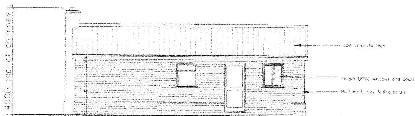
NORTH ELEVATION
