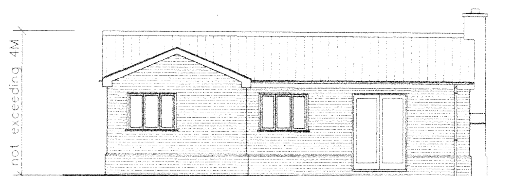
SOUTH ELEVATION
