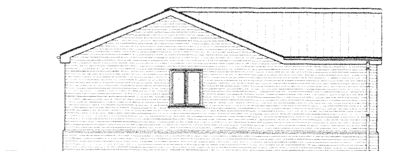
WEST ELEVATION
