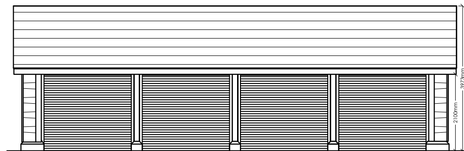
FRONT ELEV. 1:100
