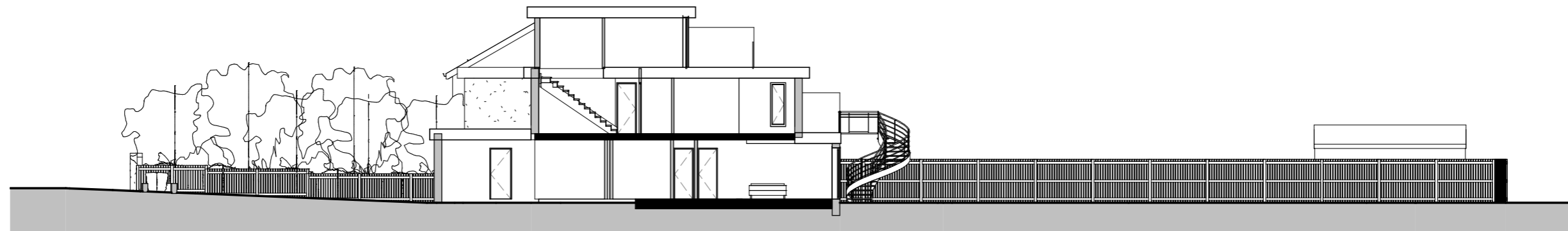
1 North South Site Section 1 : 200
