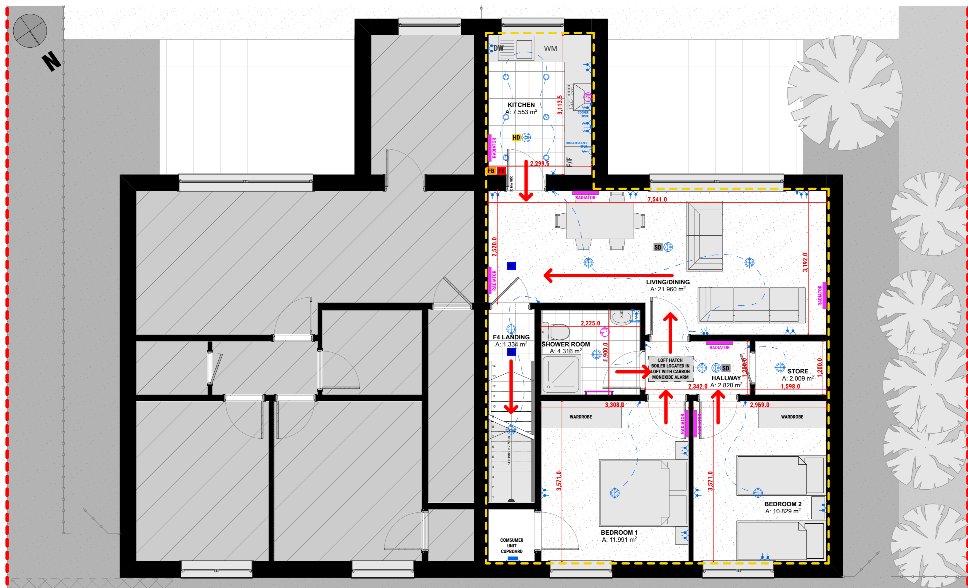
26B NETHERHILLS AVENUE APARTMENT PLAN SCALE 1:50
