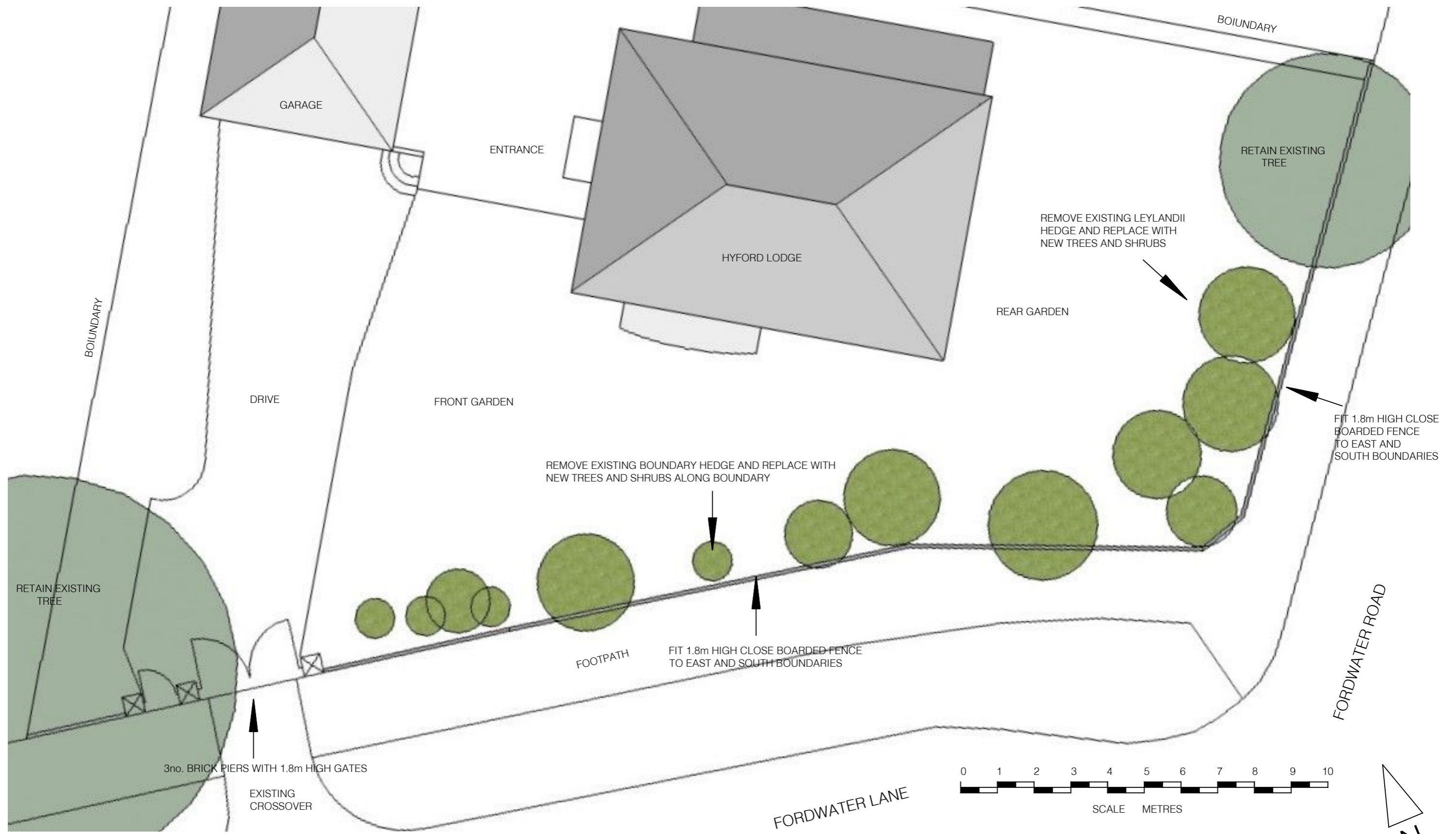
PROPOSED SITE PLAN 1:100
