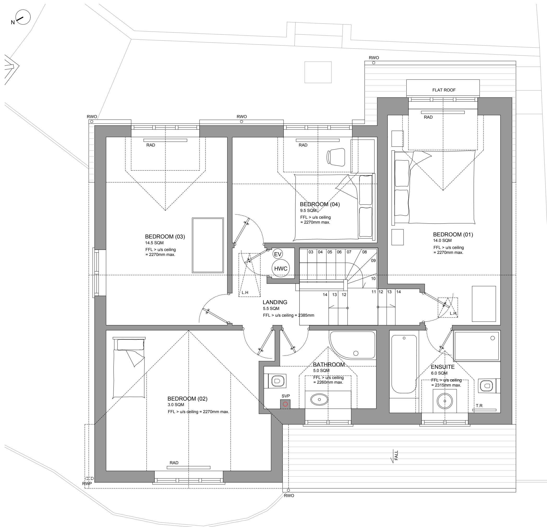
EXISTING FIRST FLOOR PLAN SCALE 1:50
