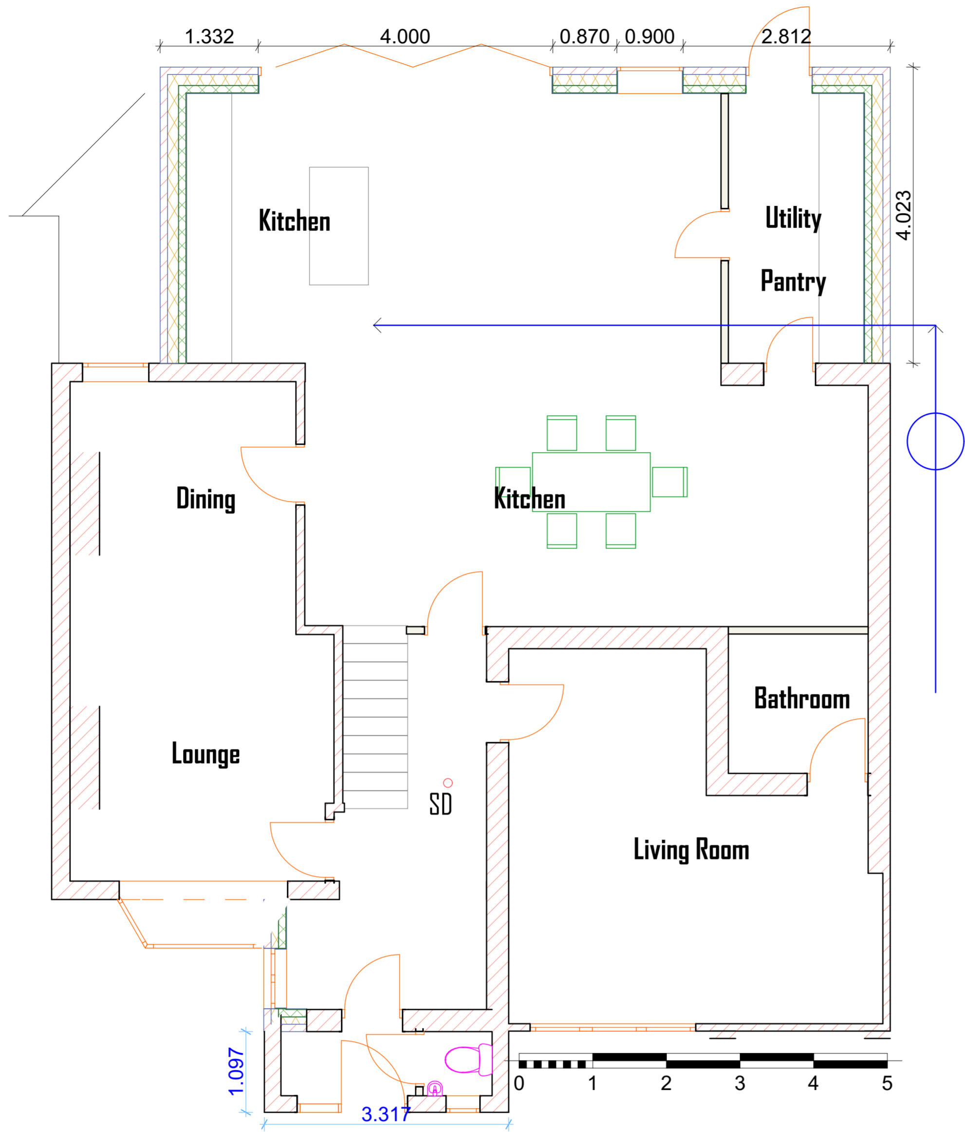
0. Ground floor 1:50
