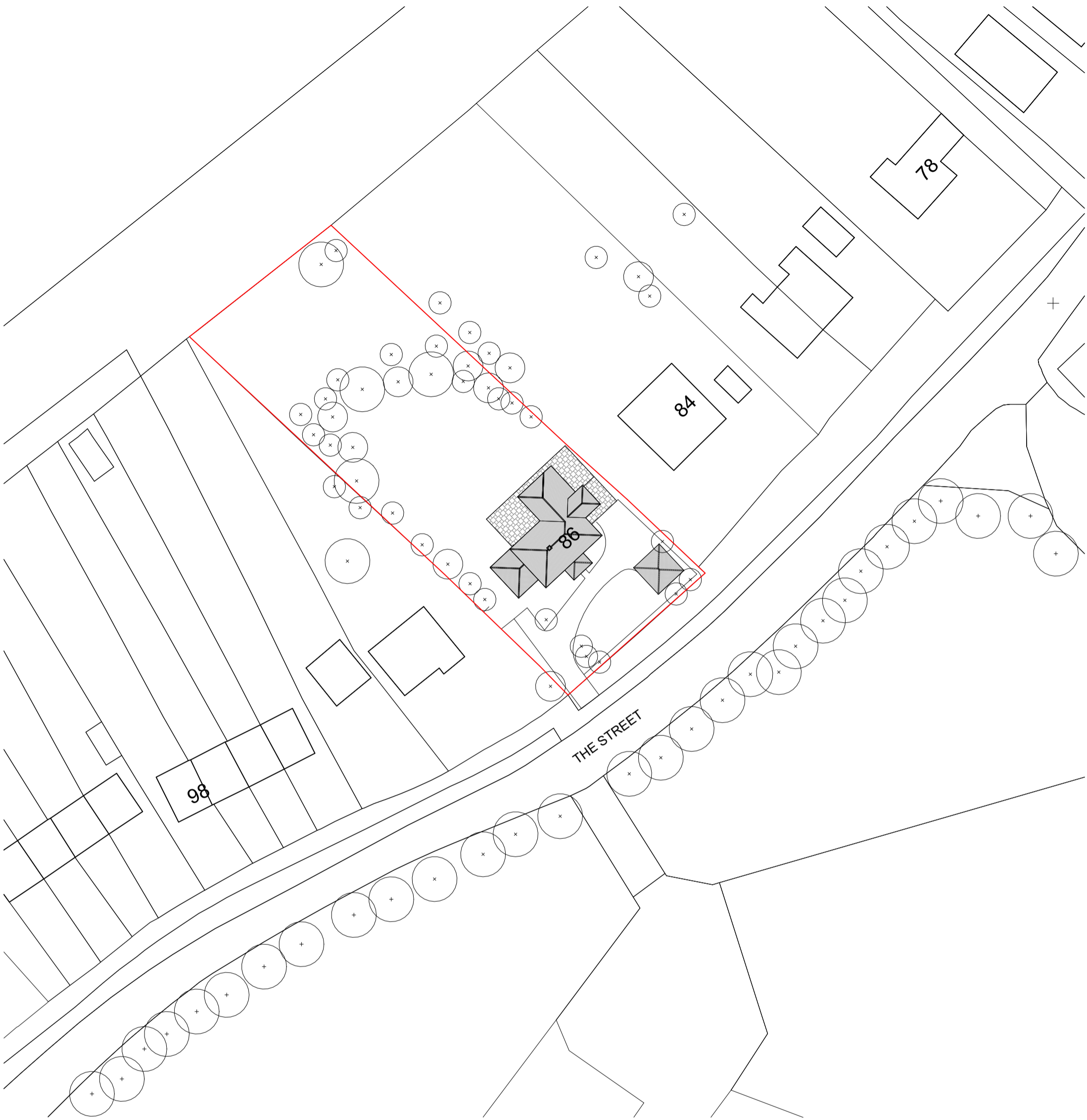
1 Proposed site plan 1 : 500
