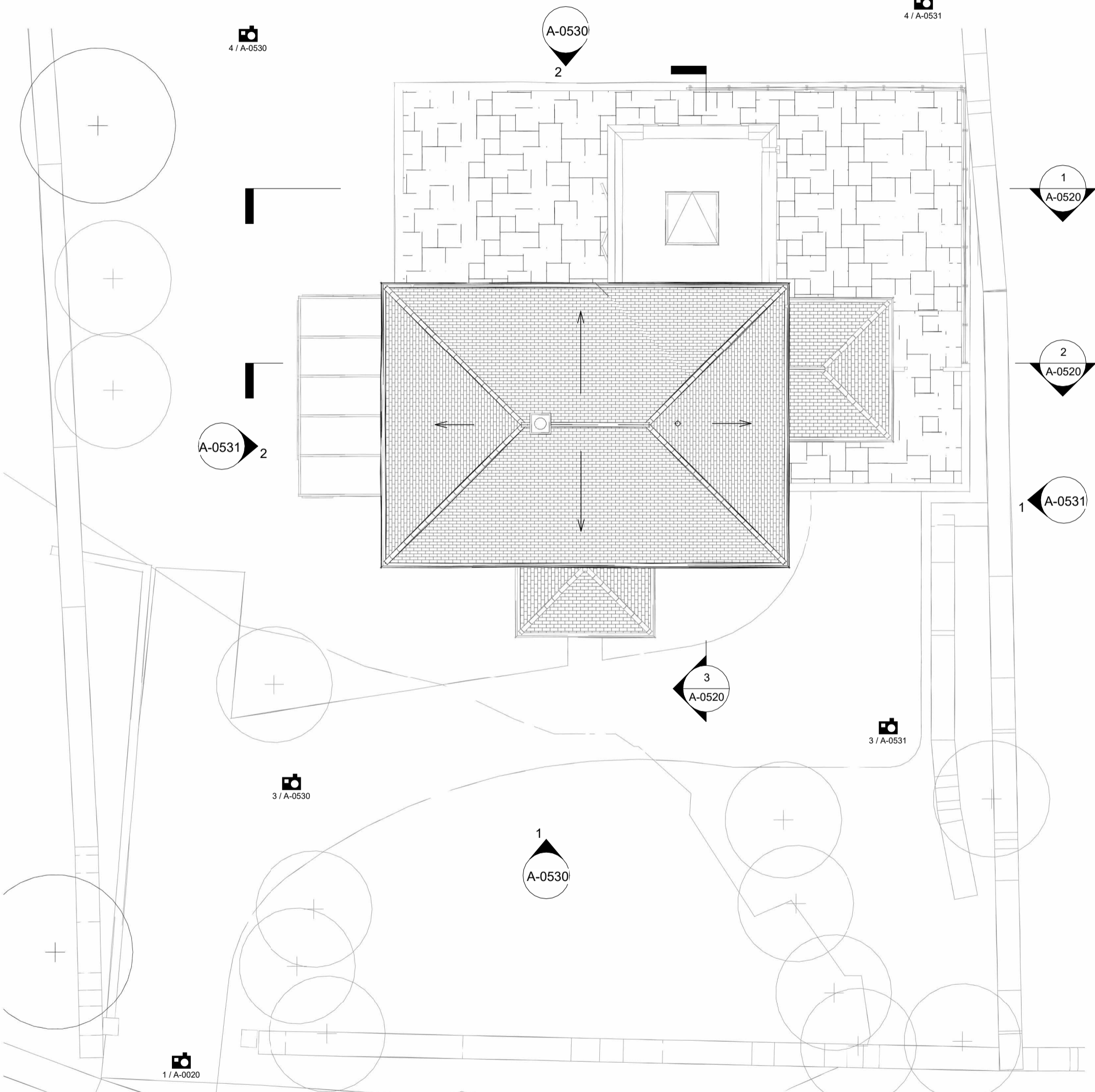
1 Existing roof plan 1 : 100
