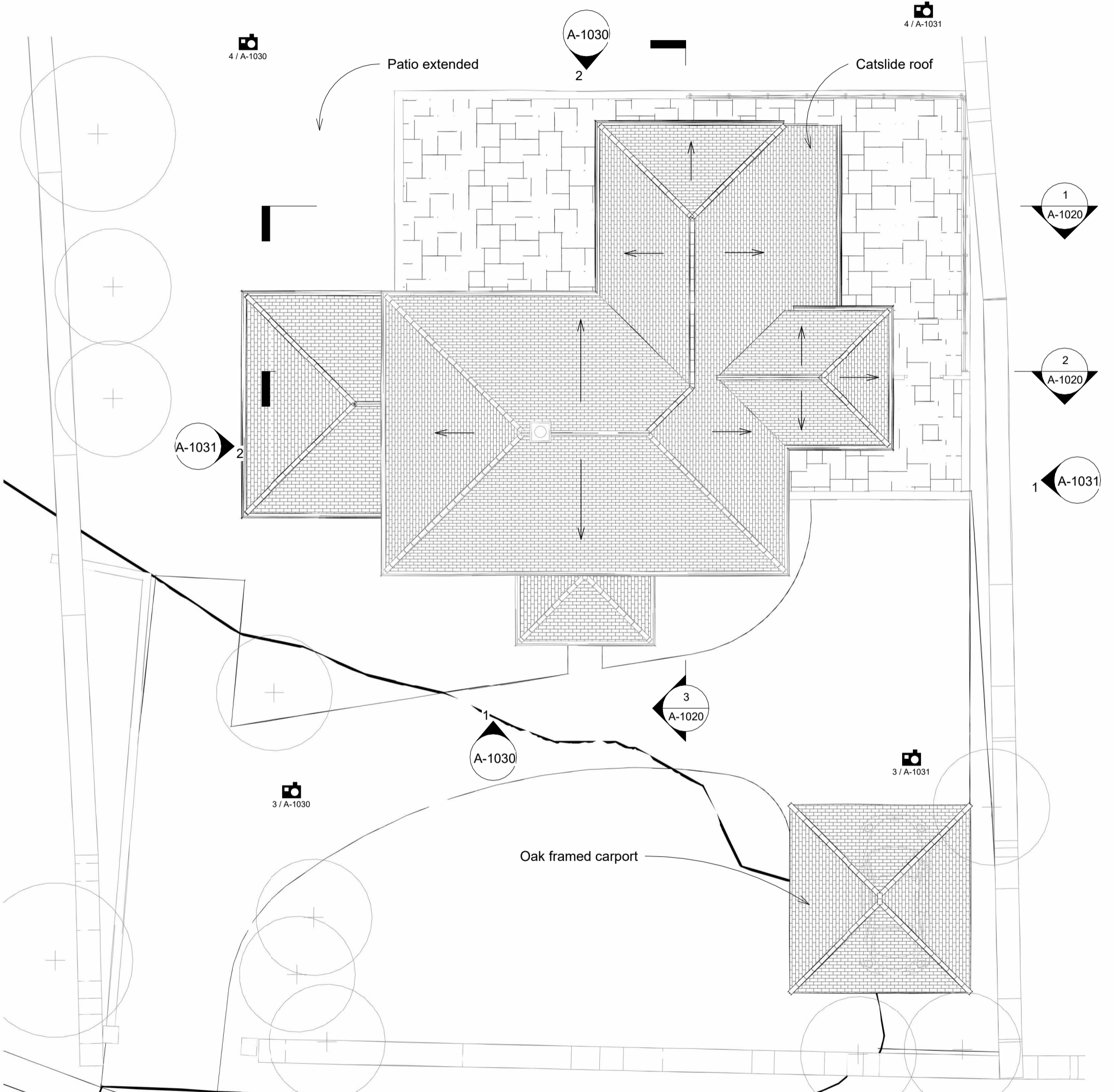
1 Proposed roof plan 1 : 100
