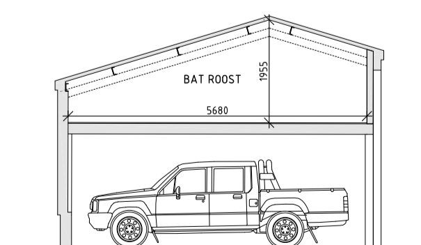
SECTION THROUGH PROPOSED BAT ROOST TO BE FORMED WITHIN ROOF VOID OF THE STABLES BLOCK. SCALE 1:100
