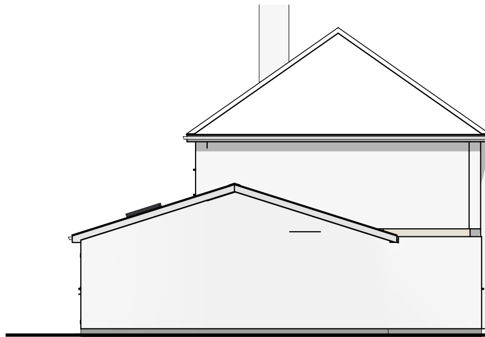
Side Elevation Scale 1:100 0 4m
