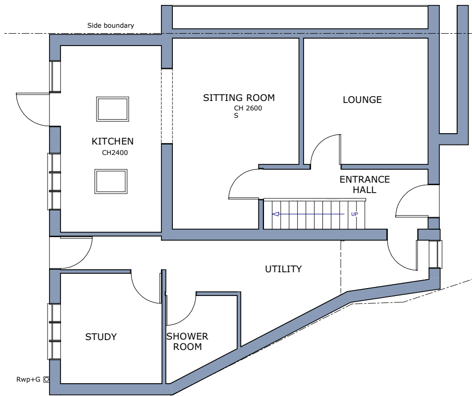
Extg. GF Plan Scale 1:100 0 4m
