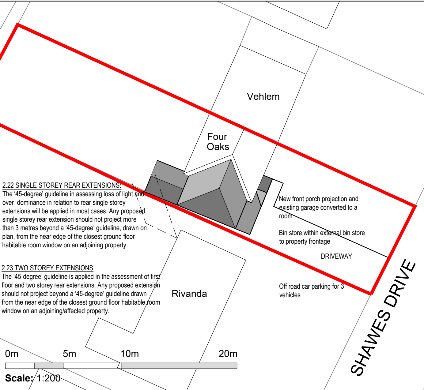
Site block plan - 1:200
