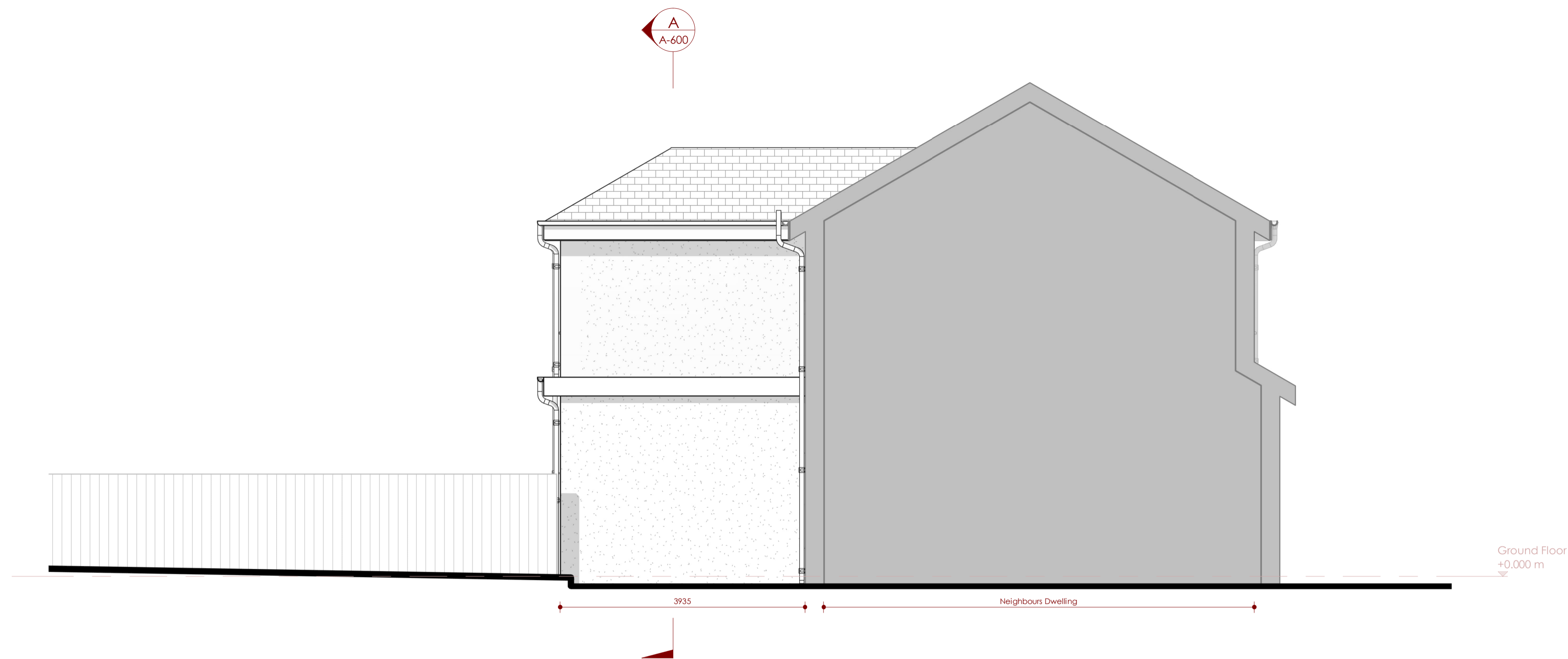
Proposed Boundary Elevation 1 : 50
