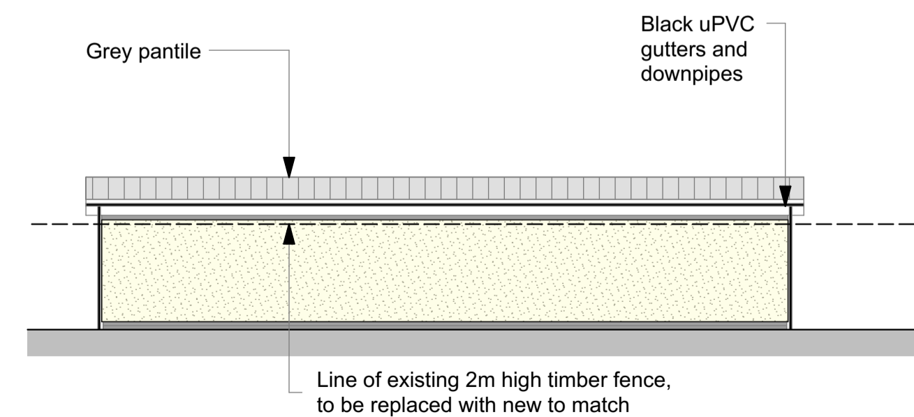
ELEVATION E-08 PROPOSED
