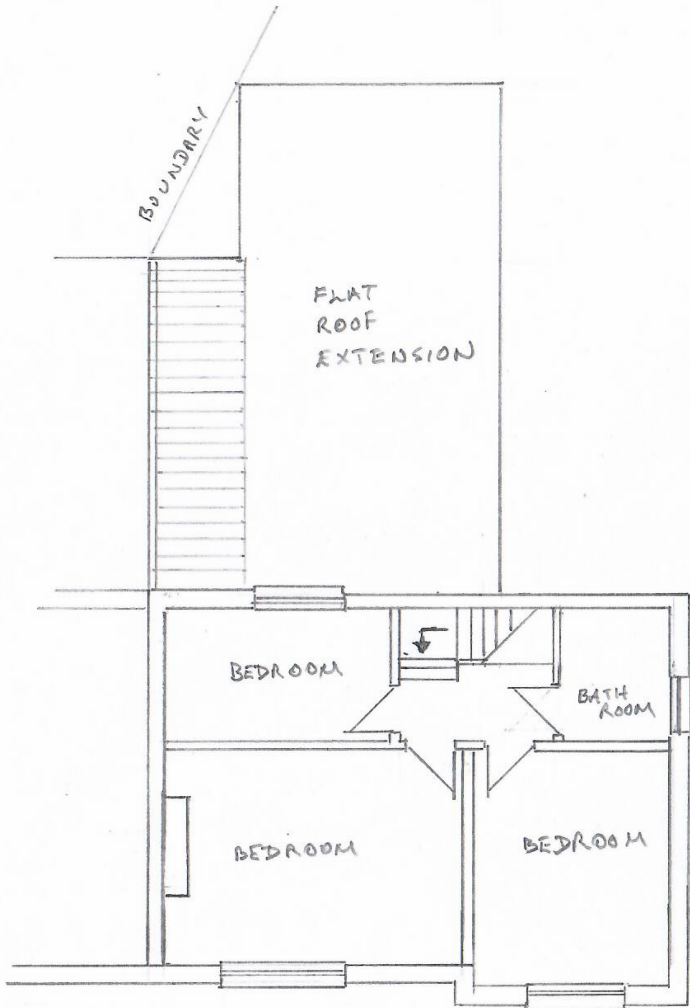
EXISTING 1st FLOOR
