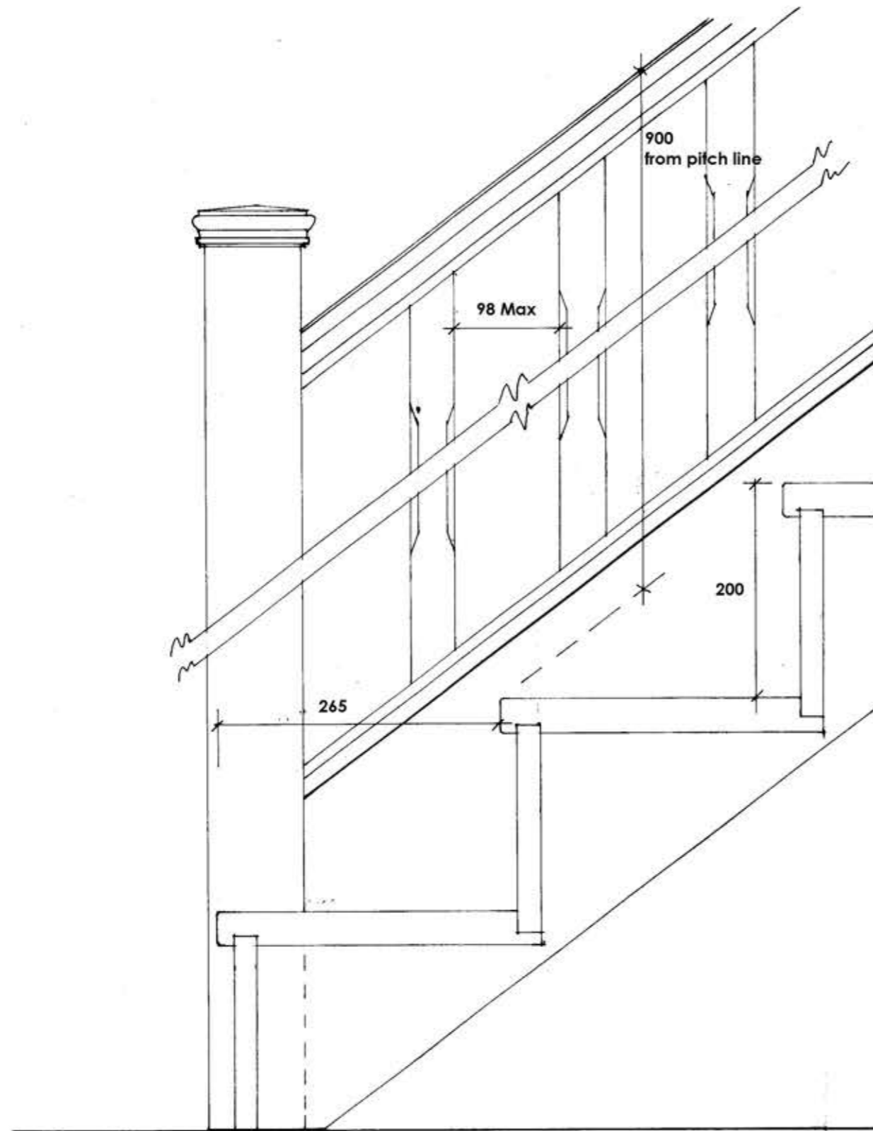
PART ELEVATION/ SECTION TO STAIR CASE
