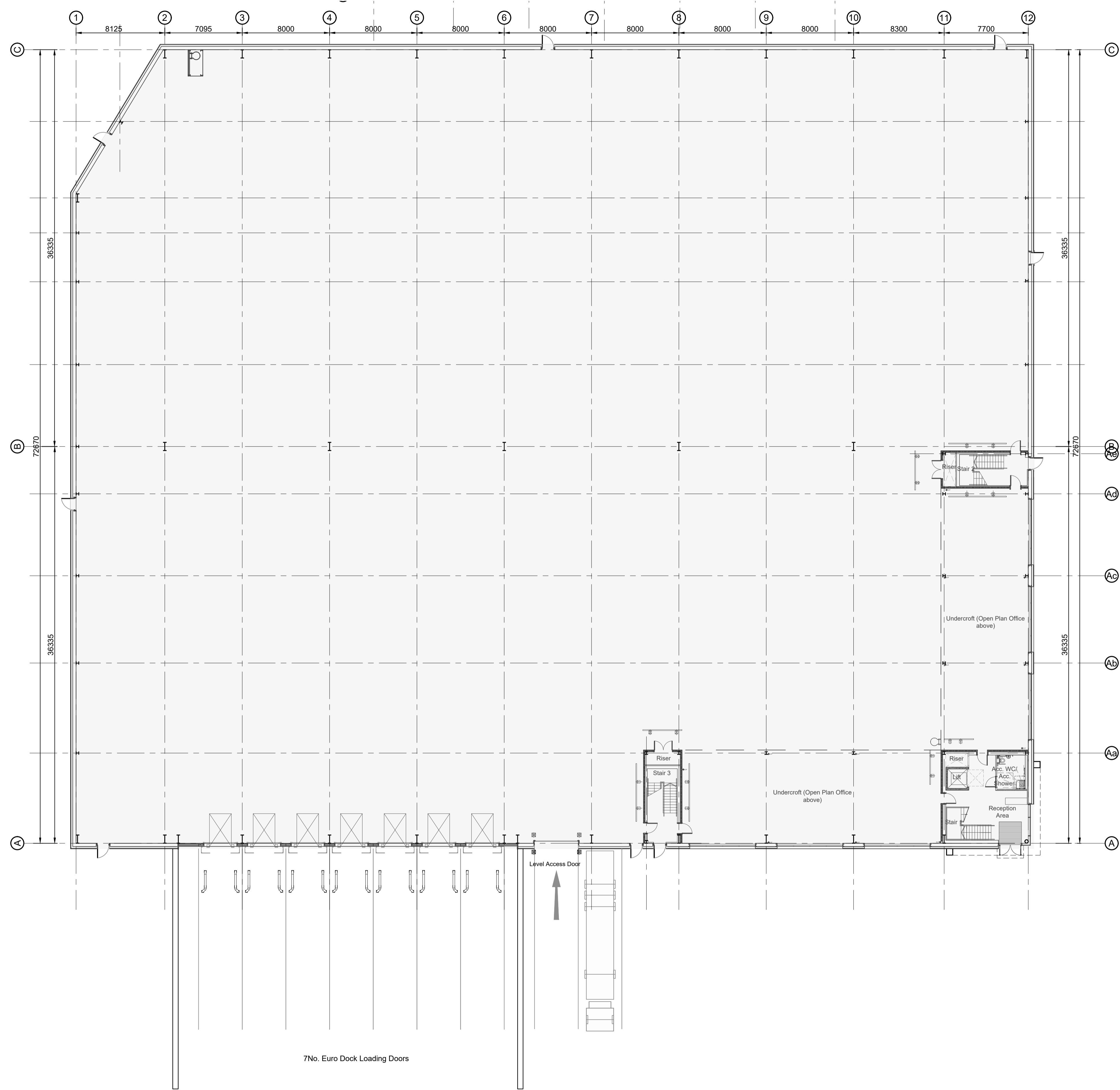
Unit 100: Building Layout Scale 1:200
