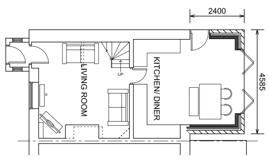
GROUND FLOOR PLAN AS PROPOSED
