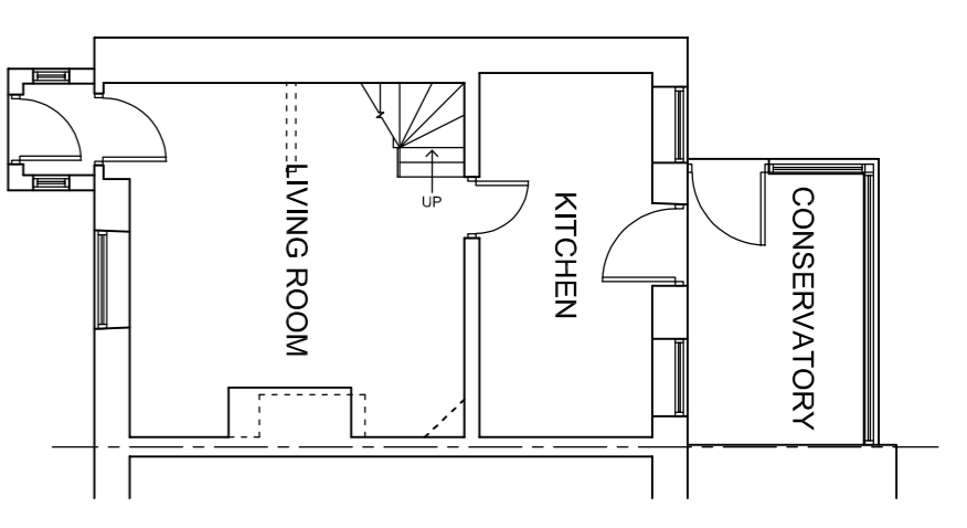
GROUND FLOOR PLAN AS EXISTING
