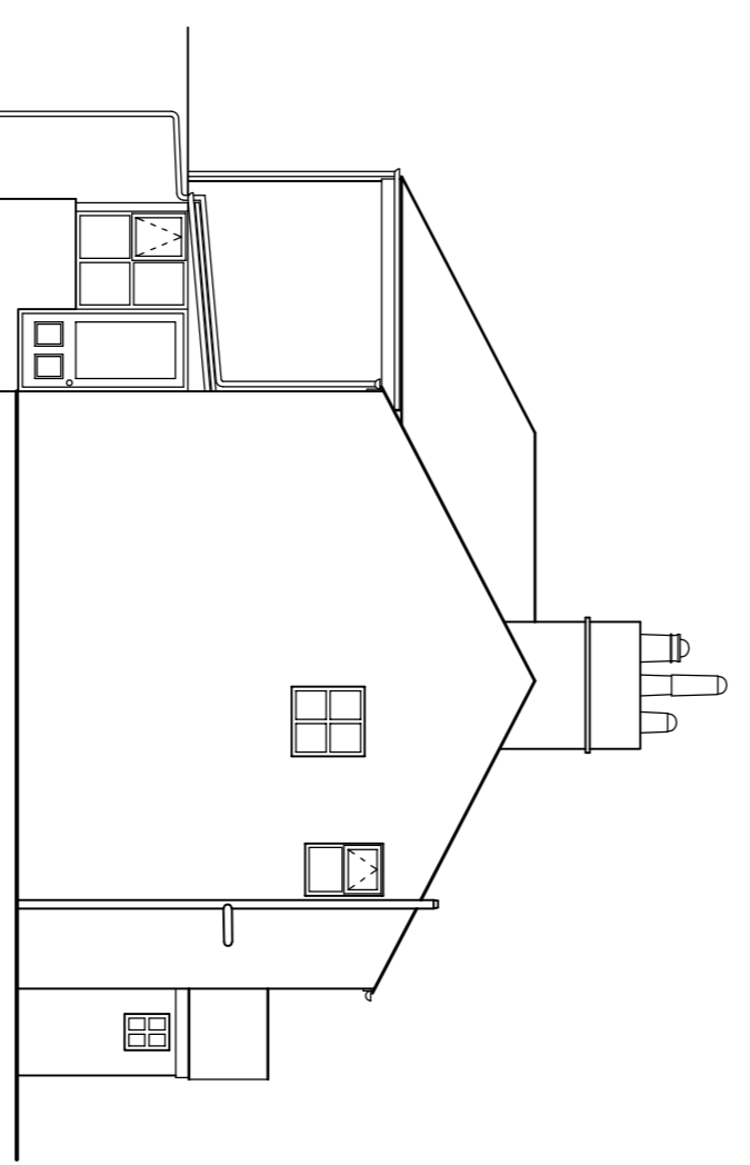
GABLE ELEVATION AS EXISTING
