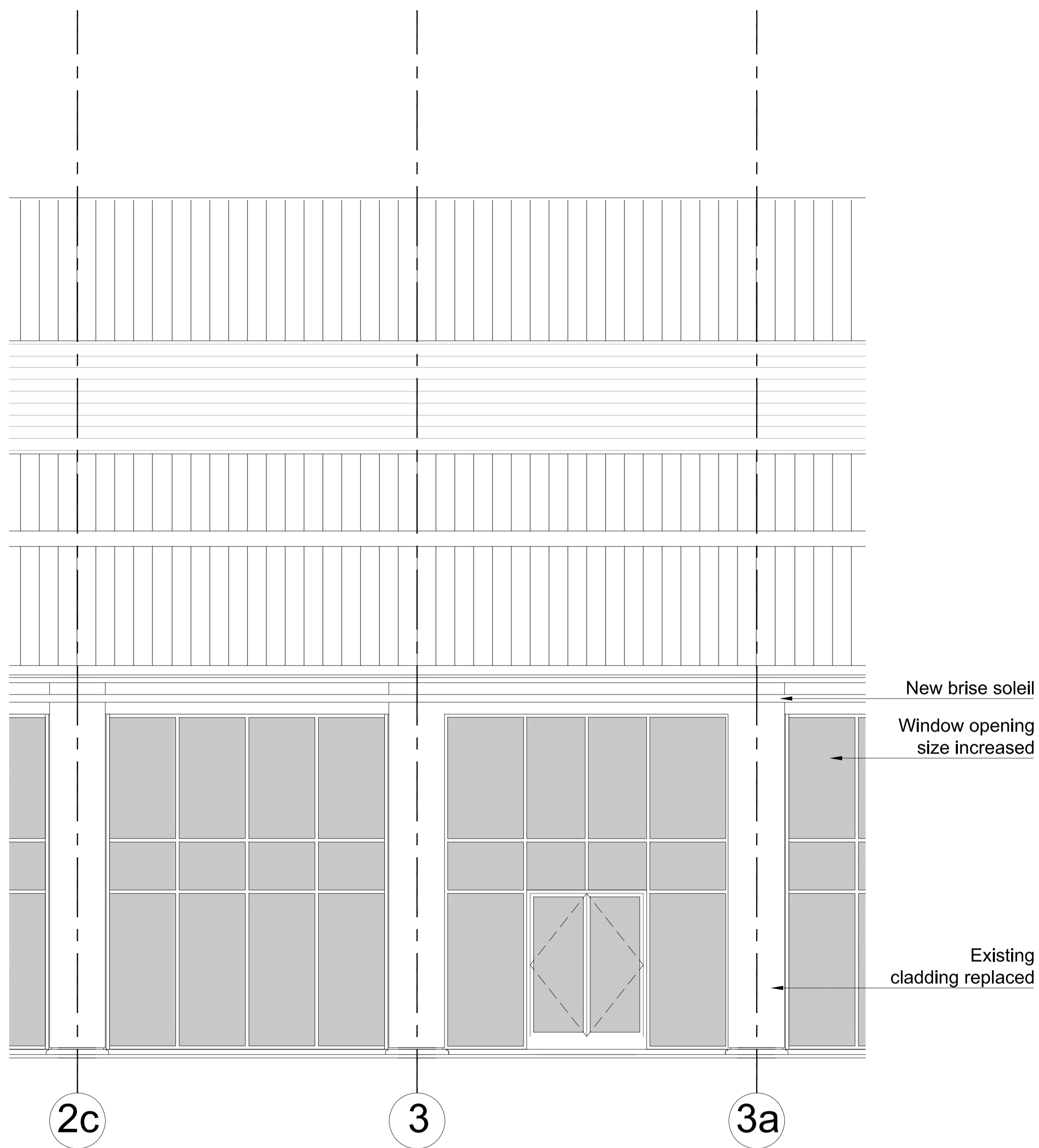
01 Bay Elevation 2 - Consented Application Scale 1:50
