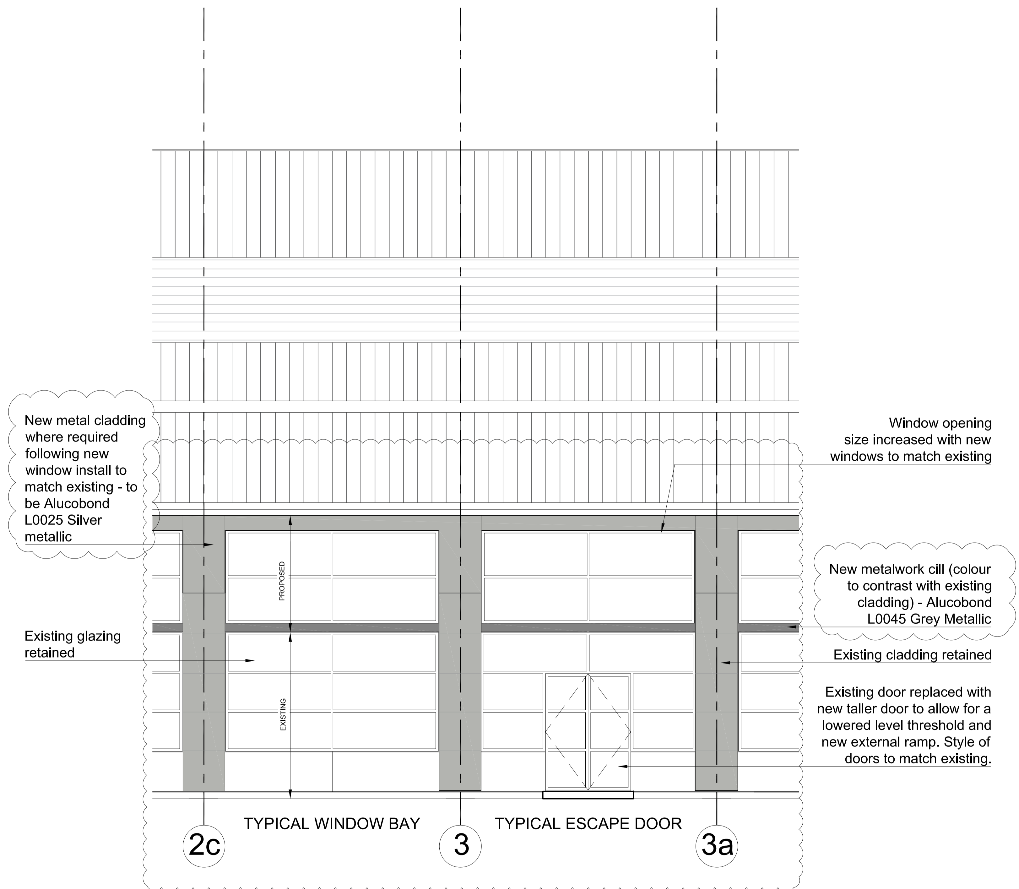
02 Bay Elevation 2 - Proposed Scale 1:50
