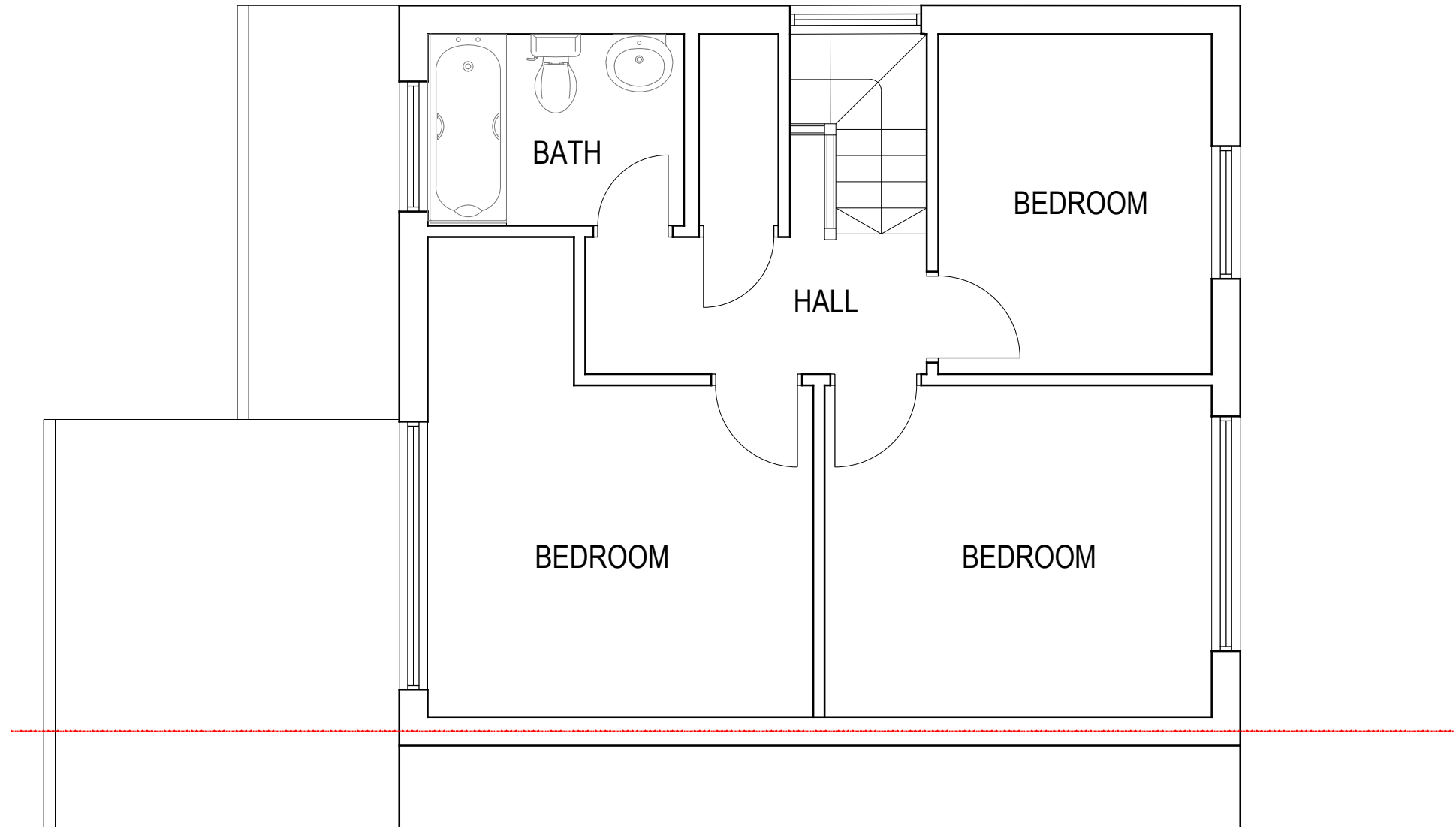
PROPOSED FIRST FLOOR PLAN (NO CHANGE)
