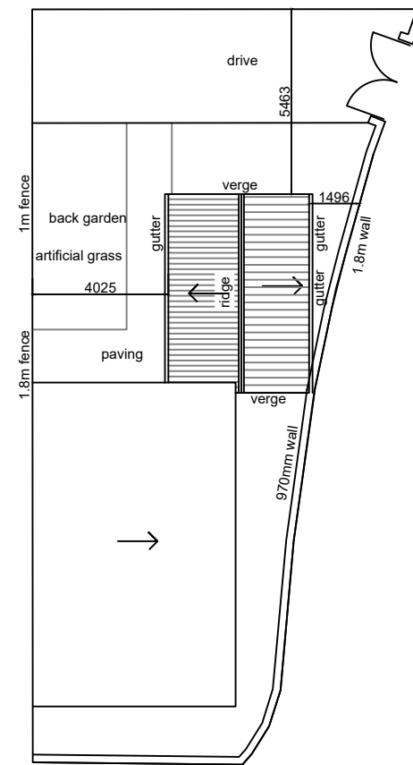
proposed site and roof plan scale 1:200
