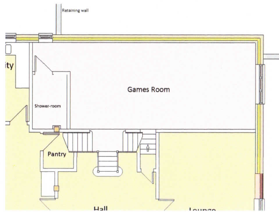
Lower Ground Floor Plan
