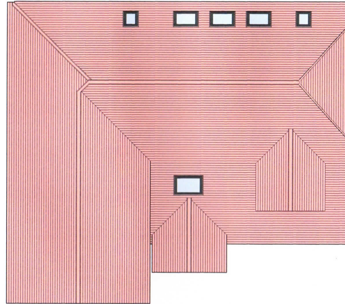
Roof plan
